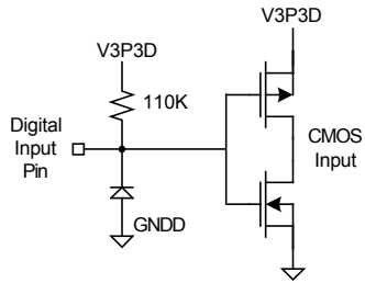
Digital Input Equivalent Circuit
