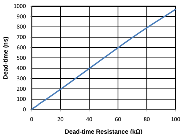
Figure 37. Dead Time vs. Resistance ( R_{DT} )
