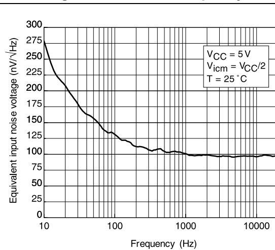
Figure 17. Noise vs. frequency
