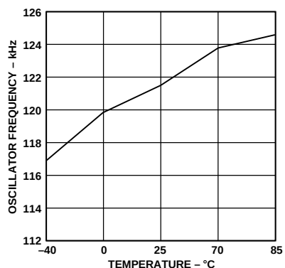
Figure 5. Oscillator Frequency vs. Temperature
