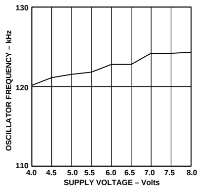
Figure 2. Oscillator Frequency vs. Supply Voltage
