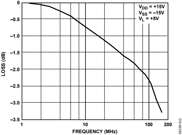
Figure 14. Frequency Response with Switch On
