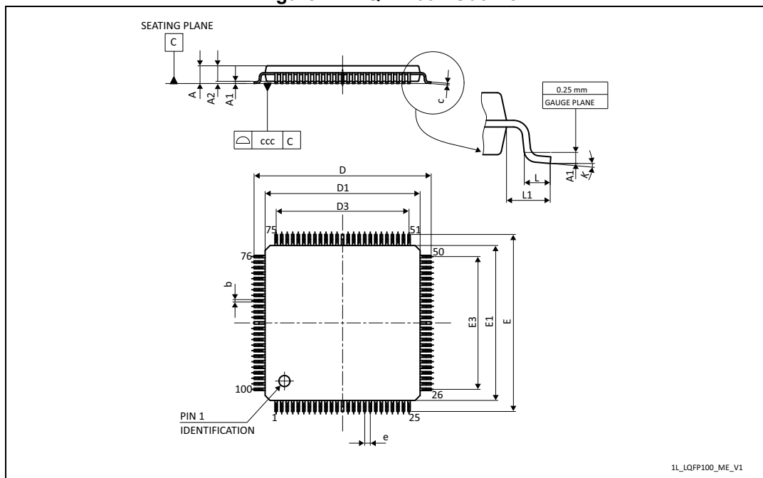
Figure 71. LQFP100 - Outline
