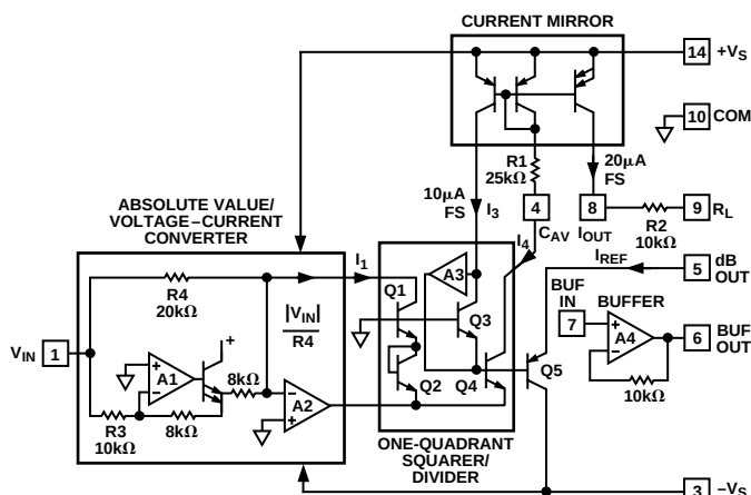
Figure 9. Simplified Schematic
