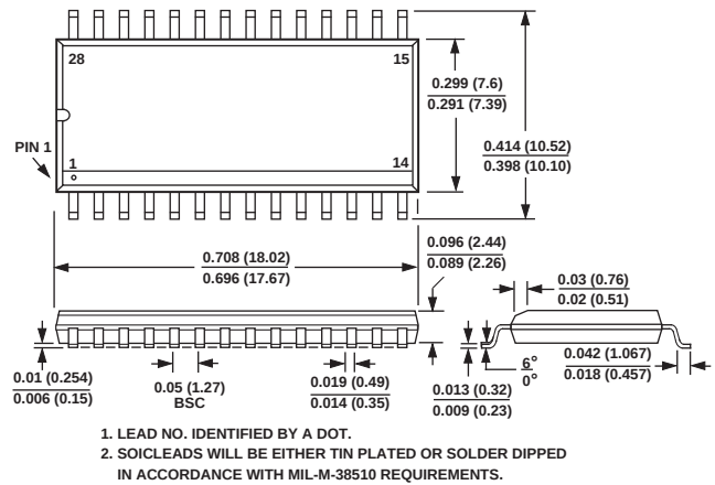
28-Lead SOIC (R-28)
