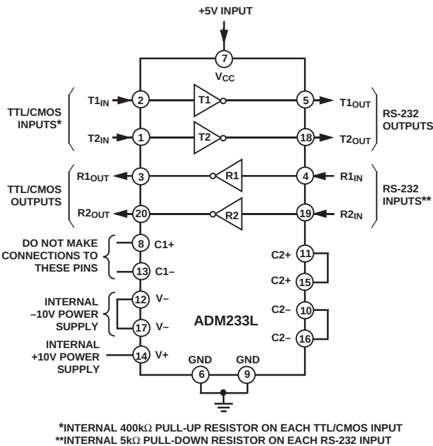
Figure 8. ADM233L Typical Operating Circuit
