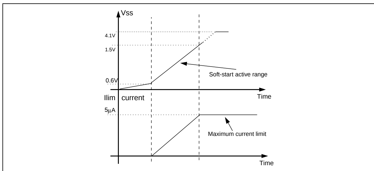
Figure 15. Soft-start diagram
