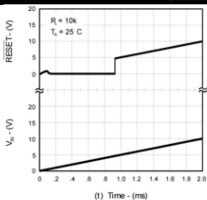
Figure 1 – Input Voltage and \overline{RESET} Output Voltage vs. Time
