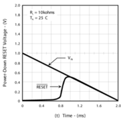
Figure 3 – Power-Down \overline{RESET} Voltage
