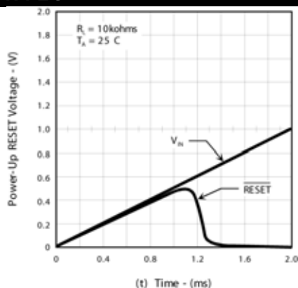
Figure 2 – Power-Up \overline{RESET} Voltage
