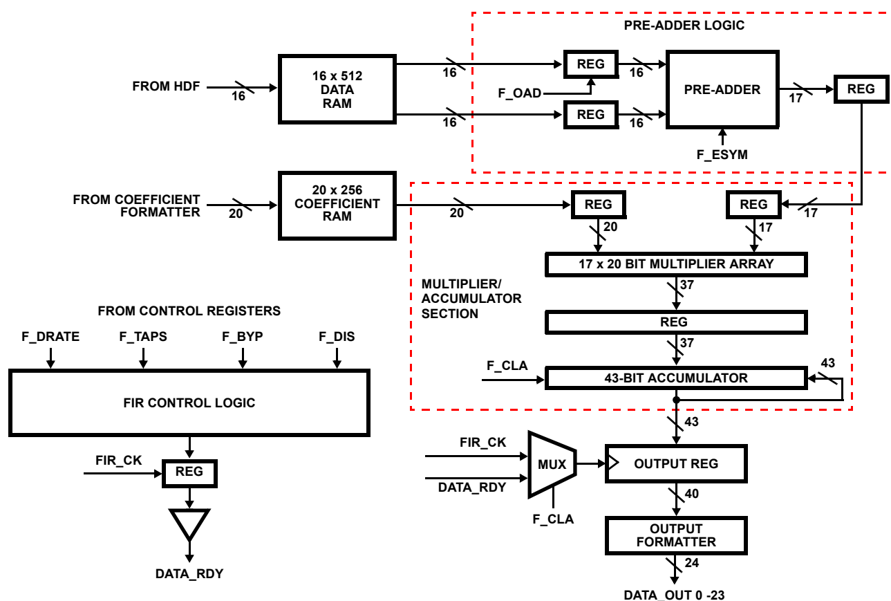
FIGURE 9. FIR FILTER
