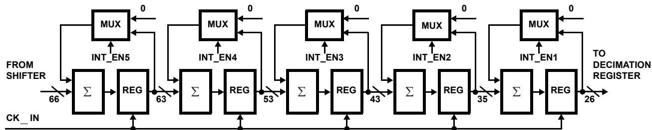
FIGURE 2. INTEGRATOR
