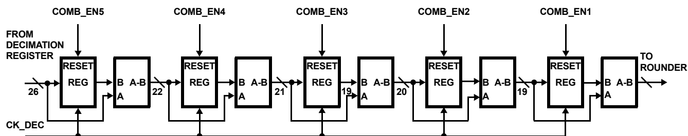
FIGURE 3. COMB FILTER
