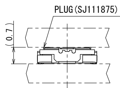
MATED CONDITION (REF.) 嵌合状態図 (参考)
