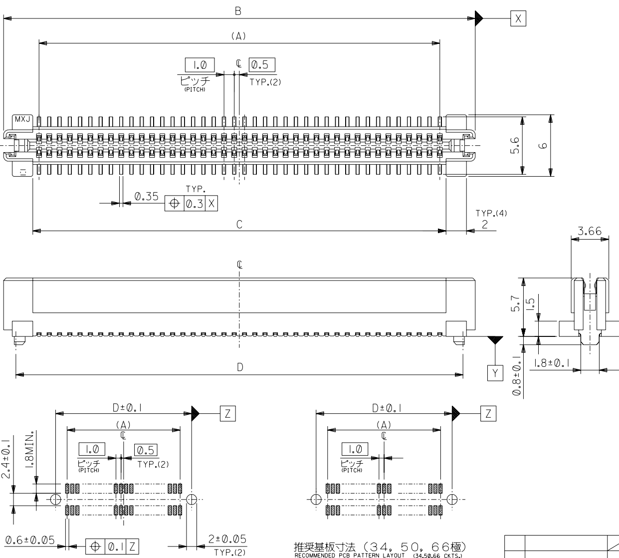
推奨基板寸法 (20, 60, 80, 84, 100, 120, 140極) RECOMMENDED PCB PATTERN LAYOUT (20,60,80,84,100,120,140 CKTS.)
