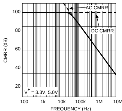
Figure 45. CMRR Curve
