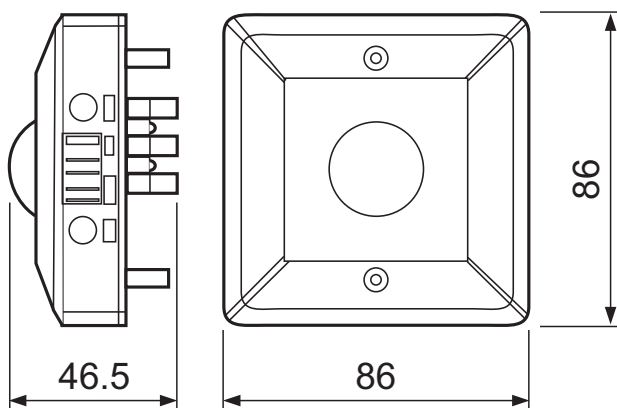
LRM1030 OS mov det switch 3 wire
