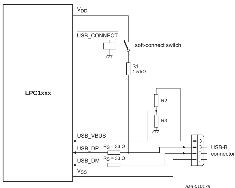
Fig 26. USB interface on a self-powered device where USB_VBUS = 5 V
