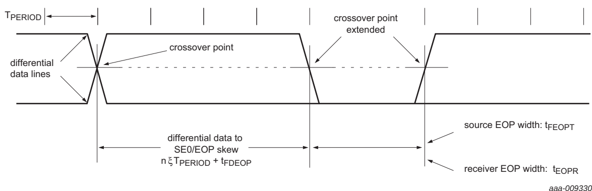
Fig 25. Differential data-to-EOP transition skew and EOP width
