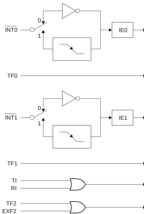
Figure 6. Interrupt Sources
