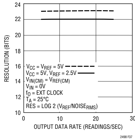
Figure 37. Resolution ( \text{Noise}_{RMS} \leq 1\text{LSB} ) vs Output Data Rate and Reference Voltage
