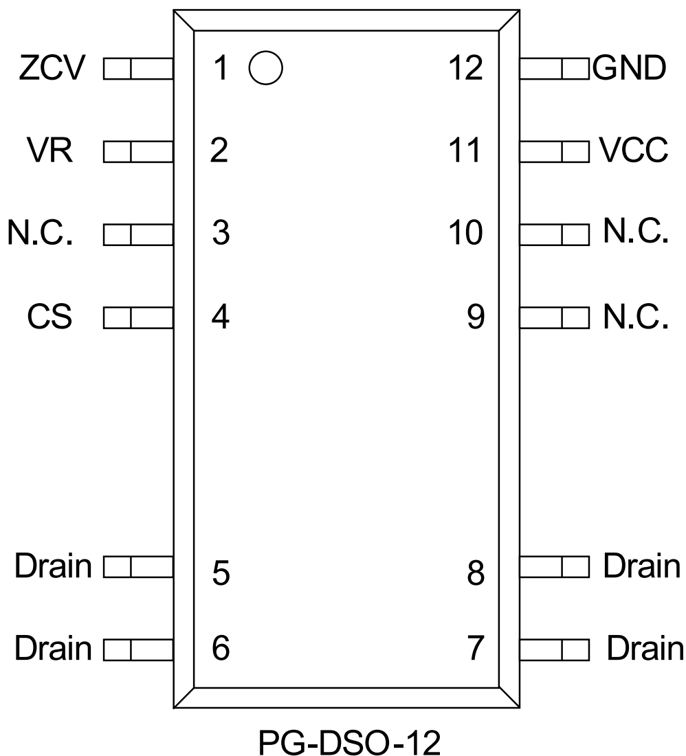
Pin Configuration PG-DSO-12 (Top View)
