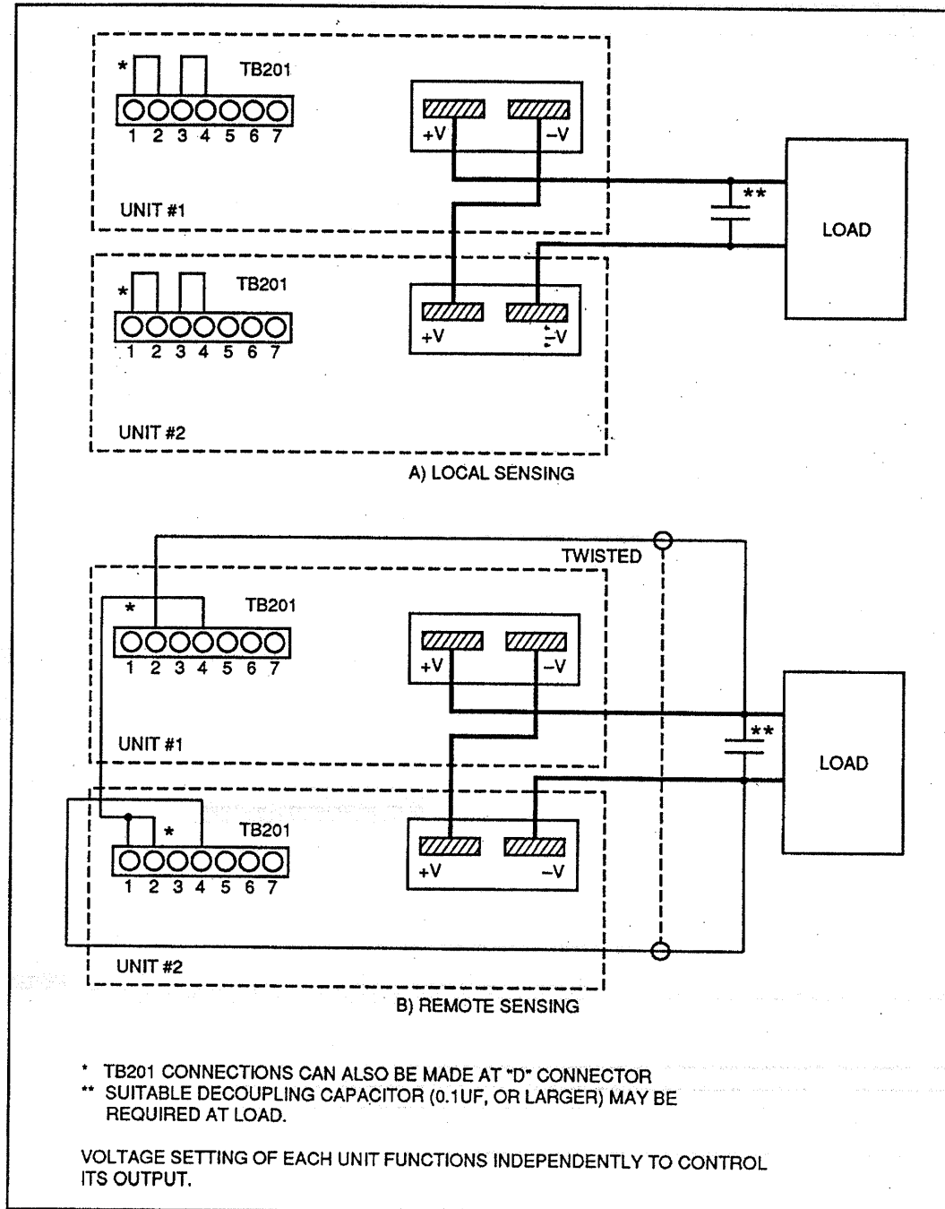
FIGURE 7: SERIES OPERATION
