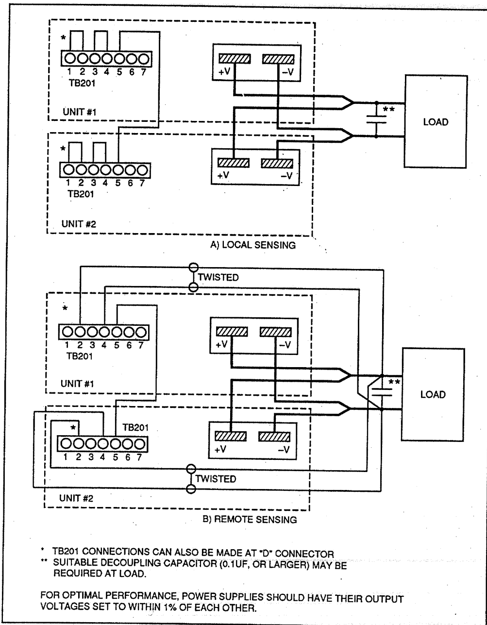
FIGURE 6: PARALLEL OPERATION
