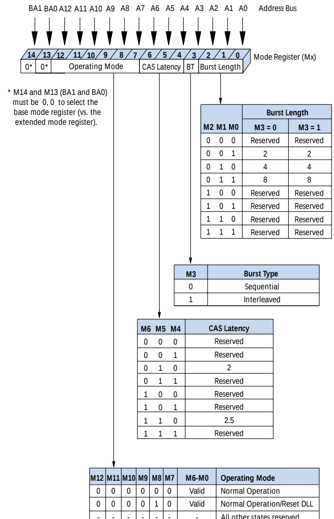
Figure 7: Mode Register Definition Diagram
