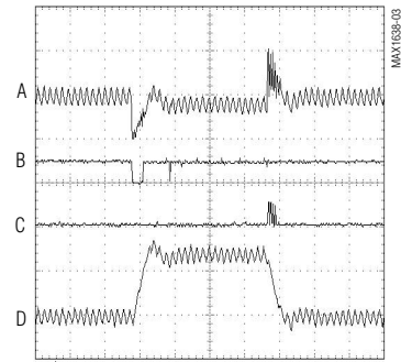
LOAD-TRANSIENT RESPONSE WITH GLITCHCATCHER
