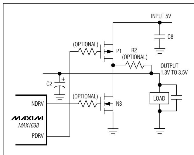
Figure 6. GlitchCatcher Circuit
