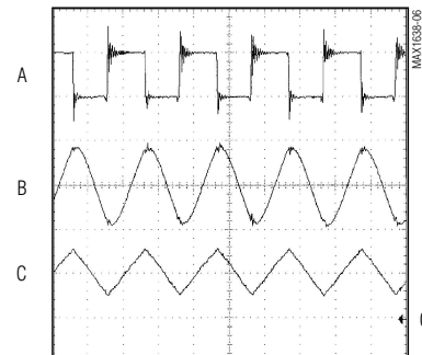
SWITCHING WAVEFORMS
