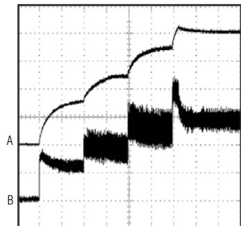
STARTUP WAVEFORMS
