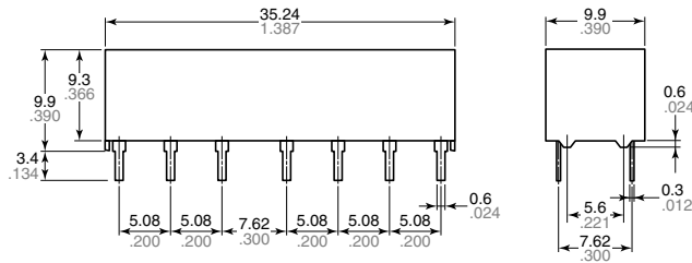
External dimensions
