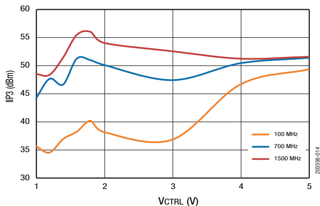
Figure 7. IIP3 vs VCTRL over Frequency (1 MHz tone spacing, +22 dBm/line)
