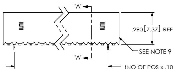
FIG 1 -SV: SINGLE VERTICAL ROW (SSM-1XX-XXX-SV-LC SHOWN)
