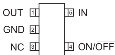
SOT23-5 (SOT25) (Top View)
