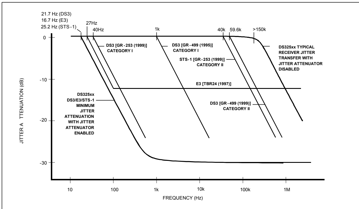
Figure 8-7. Jitter Attenuation/Jitter Transfer
