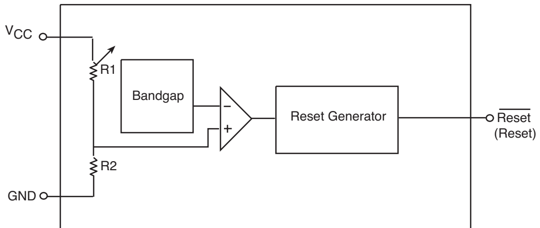
Push-Pull Type
