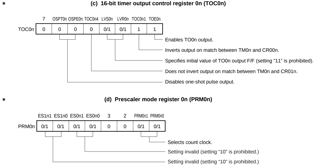
Figure 6-34. Control Register Settings in Square-Wave Output Mode (2/2)
