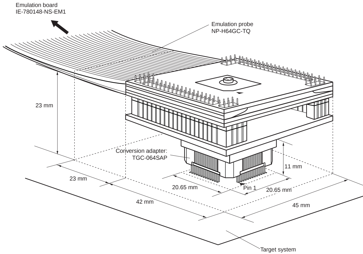
Figure B-5. Connection Conditions of Target System (When Using NP-H64GC-TQ)
