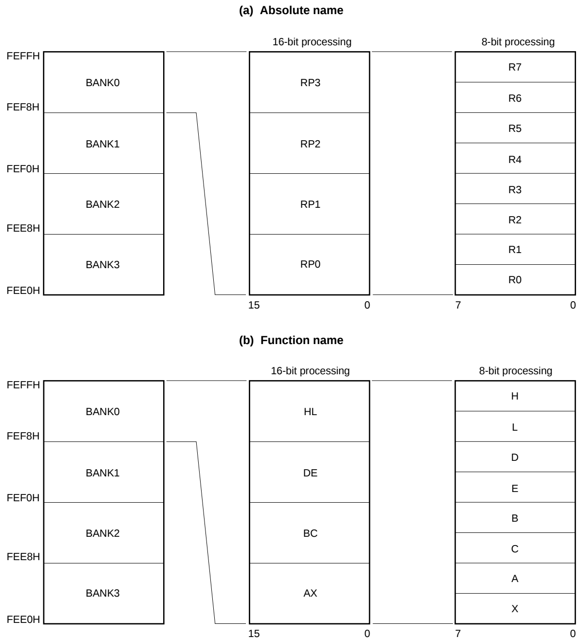
Figure 3-22. Configuration of General-Purpose Registers
