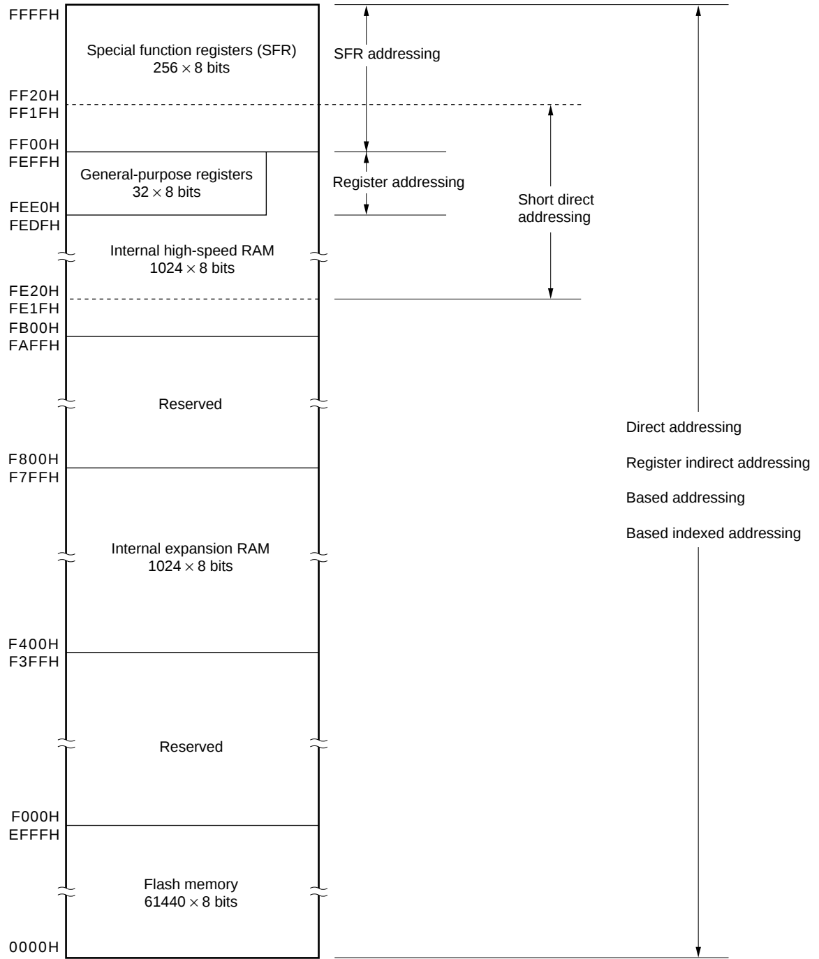
Figure 3-16. Correspondence Between Data Memory and Addressing ( \mu PD78F0138)
