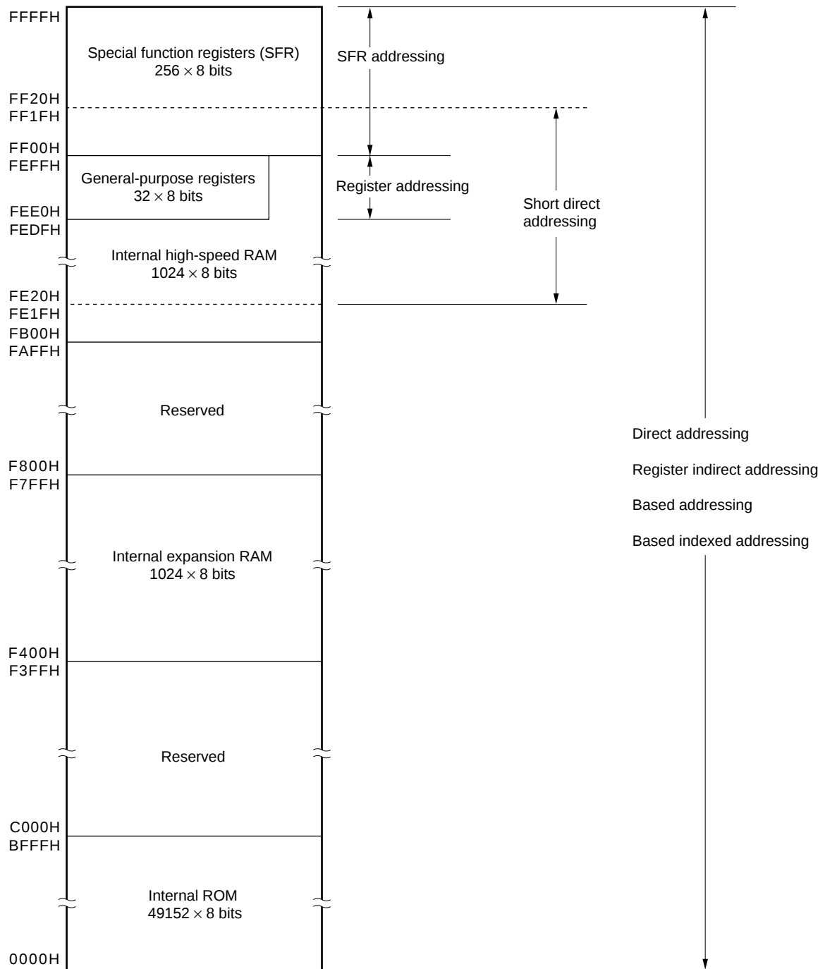
Figure 3-14. Correspondence Between Data Memory and Addressing ( \mu PD780136)
