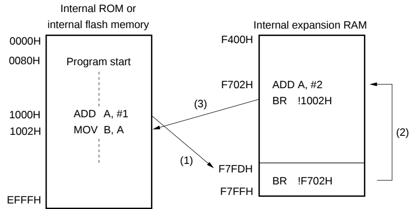
Figure 26-4. ROM Correction Usage Example
