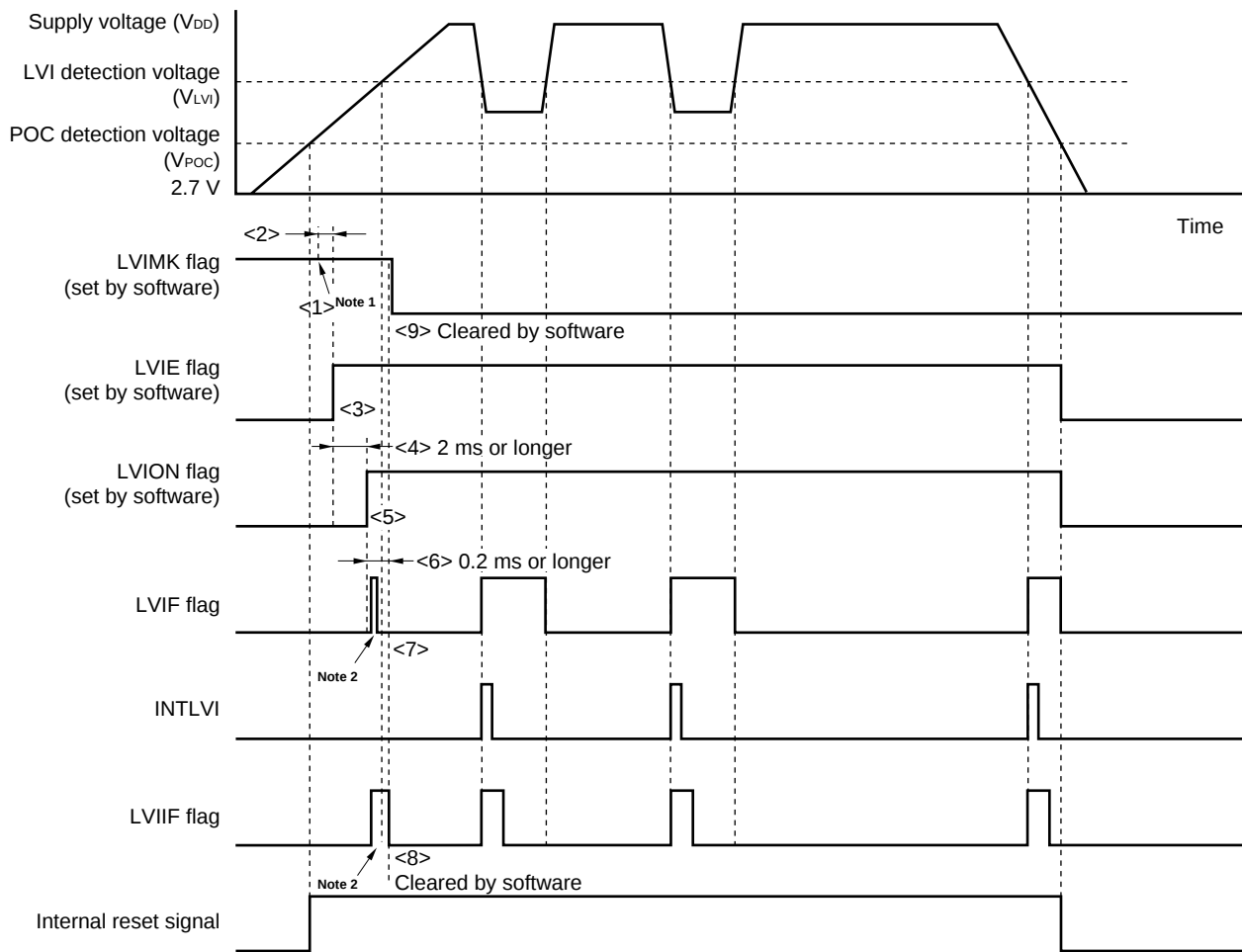
Figure 23-5. Timing of Low-Voltage Detector Interrupt Signal Generation
