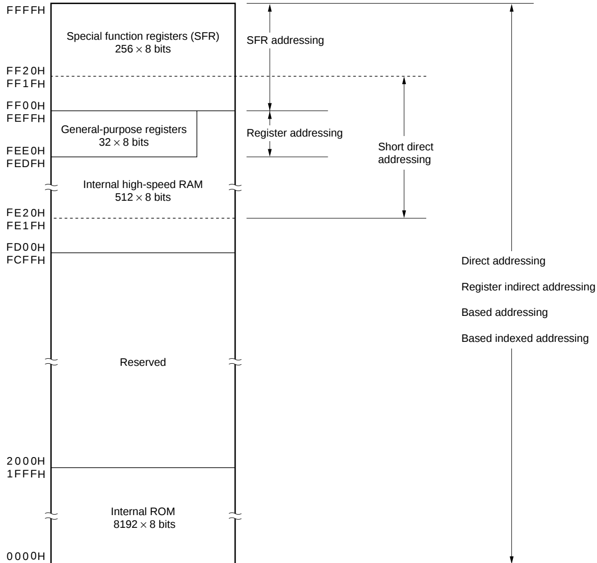
Figure 3-9. Correspondence Between Data Memory and Addressing ( \mu PD780131)
