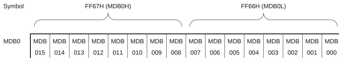
Figure 16-4. Format of Multiplication/Division Data Register B0 (MDB0)
