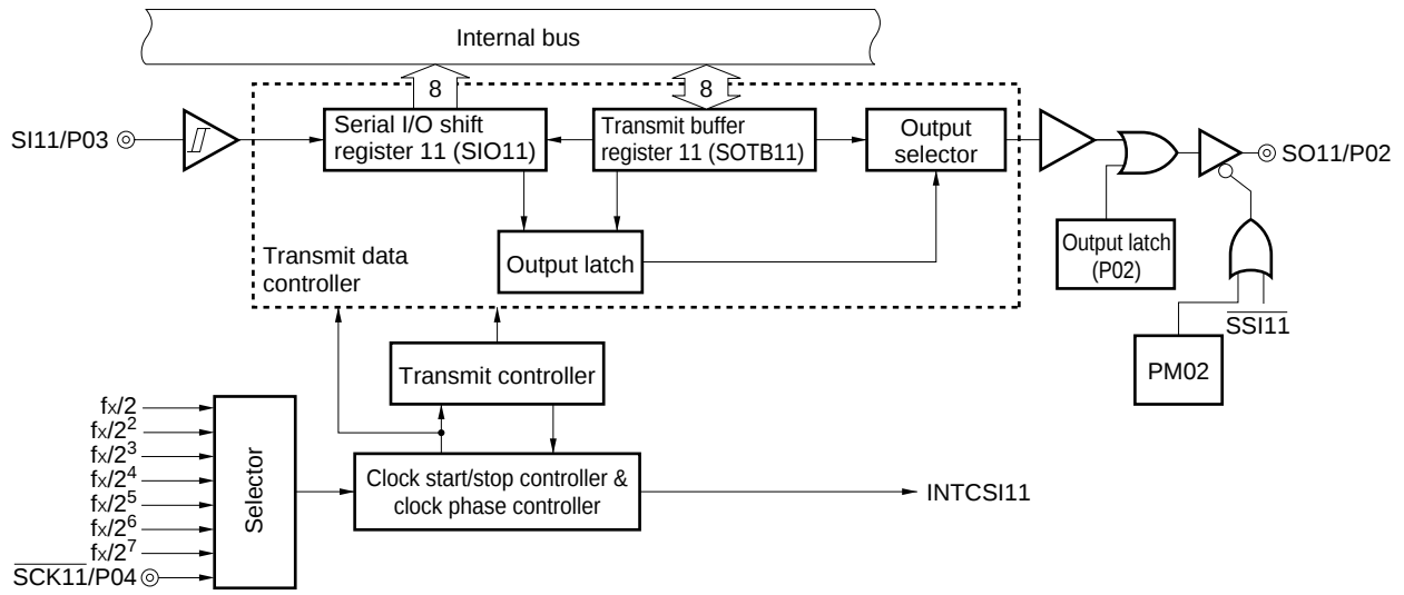
Figure 15-2. Block Diagram of Serial Interface CSI11
