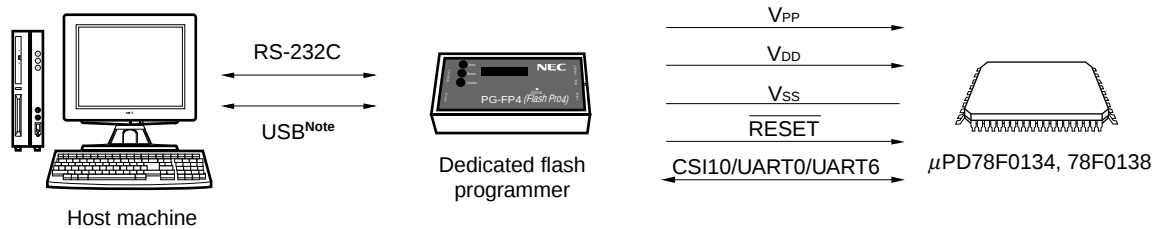
Figure 27-8. Environment for Writing Program to Flash Memory
