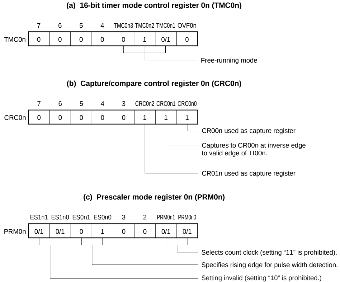
Figure 6-27. Control Register Settings for Pulse Width Measurement with Free-Running Counter and Two Capture Registers (with Rising Edge Specified)
