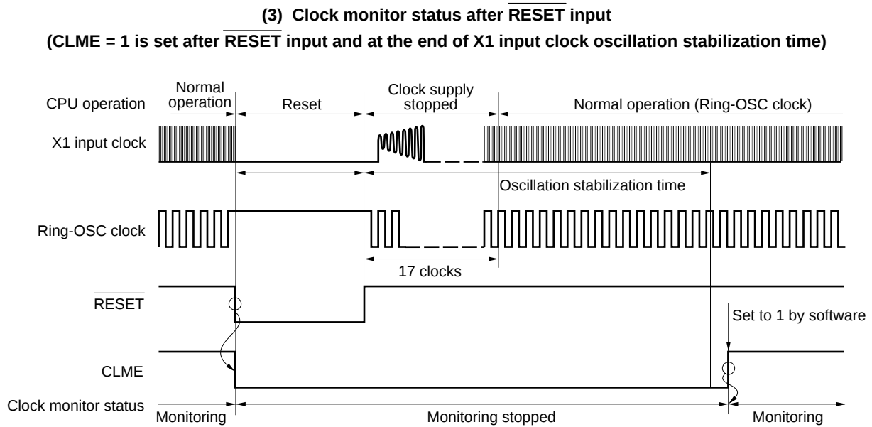
Figure 21-3. Timing of Clock Monitor (2/4)
