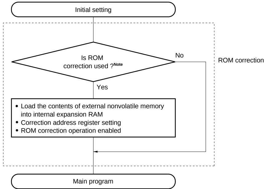
Figure 26-6. Initial Setting Routine
