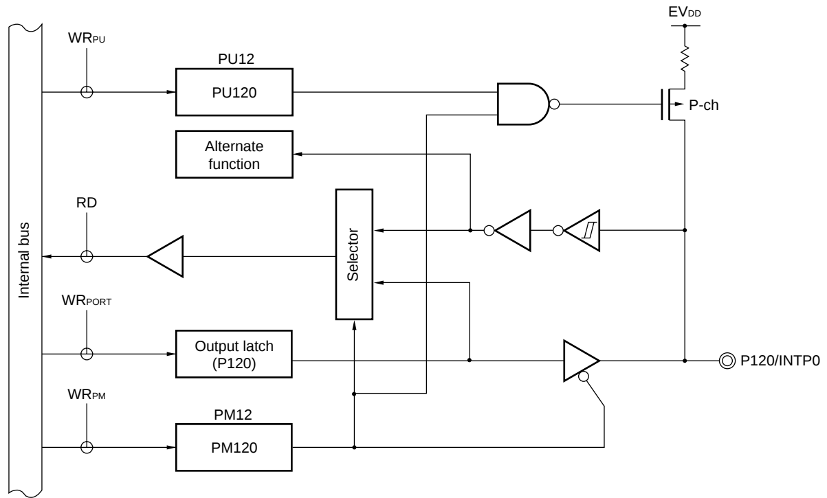
Figure 4-18. Block Diagram of P120
