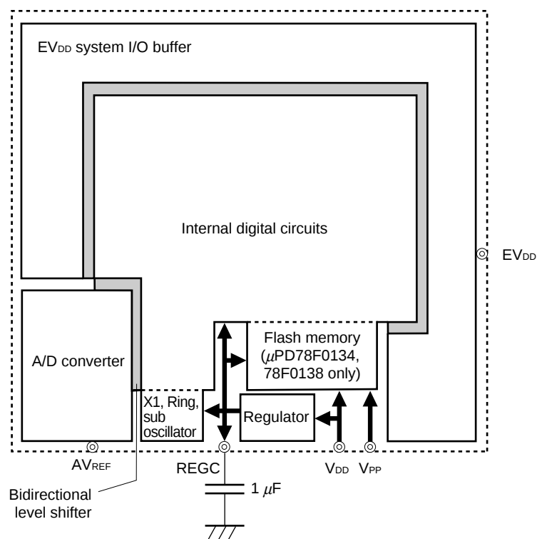
Figure 24-1. Block Diagram of Regulator Periphery
