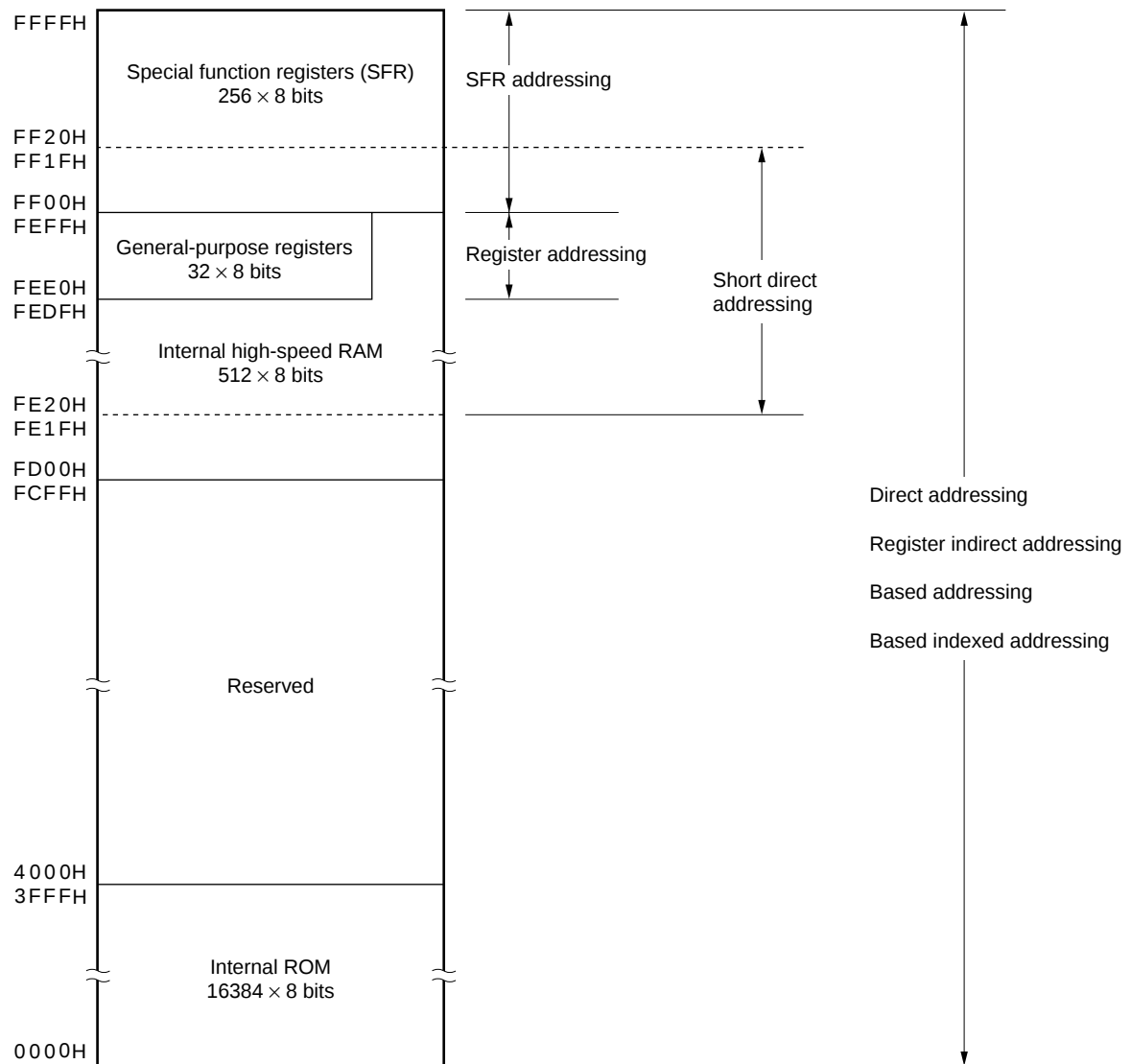
Figure 3-10. Correspondence Between Data Memory and Addressing ( \mu PD780132)
