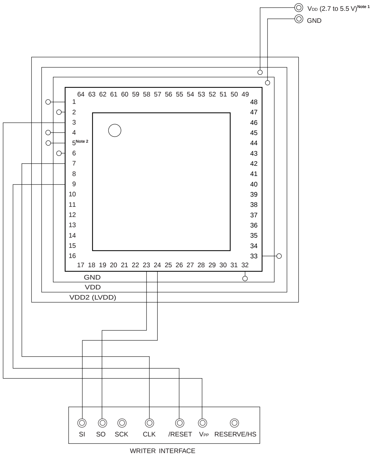
Figure 27-7. Example of Wiring Adapter for Flash Memory Writing in UART (UART6) Mode
