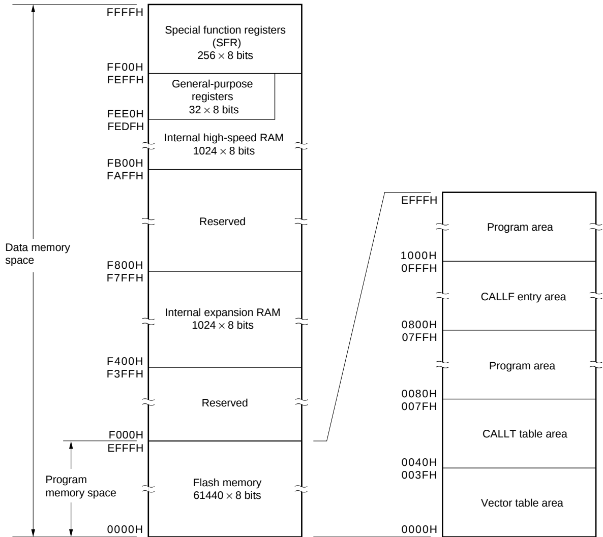
Figure 3-8. Memory Map ( \mu PD78F0138)
