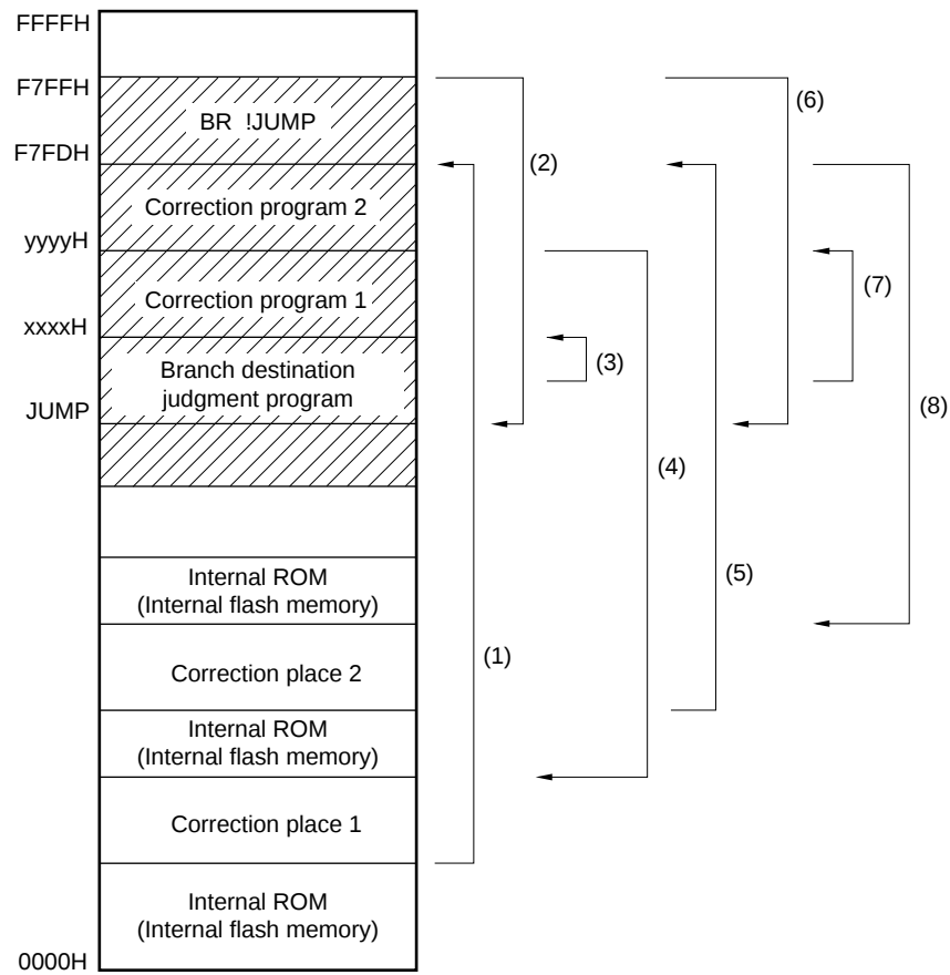
Figure 26-9. Program Transition Diagram (When Two Places Are Corrected)
