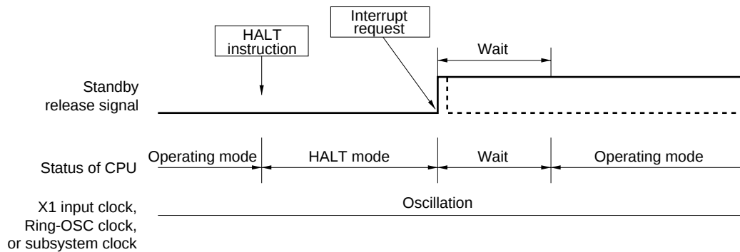
Figure 19-3. HALT Mode Release by Interrupt Request Generation
