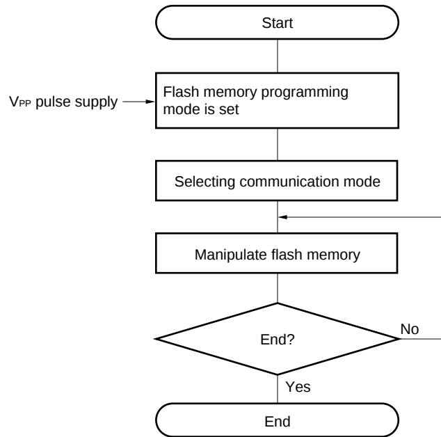
Figure 27-18. Flash Memory Manipulation Procedure
