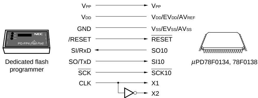
Figure 27-9. Communication with Dedicated Flash Programmer (CSI10)
