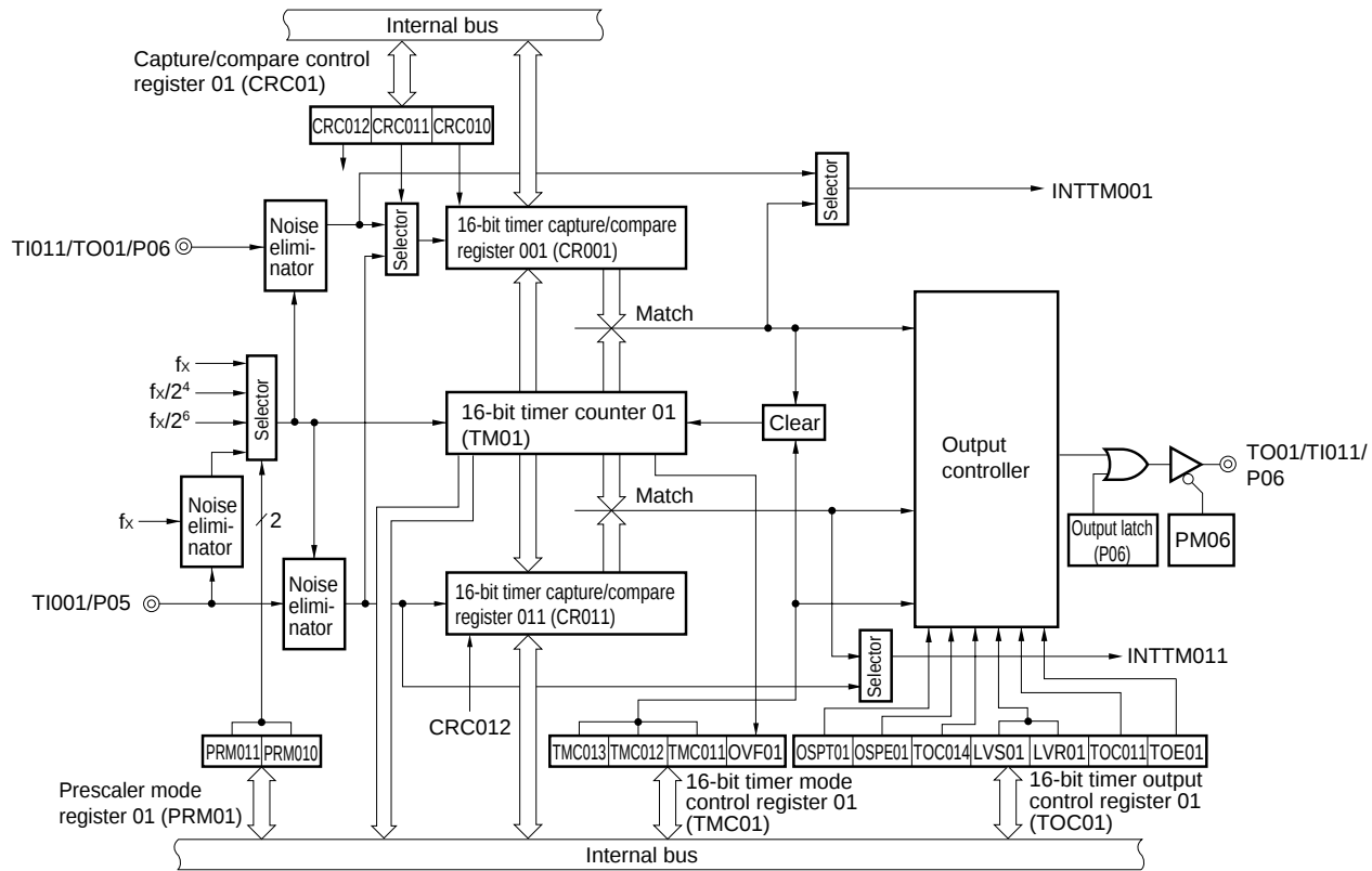
Figure 6-2. Block Diagram of 16-Bit Timer/Event Counter 01
