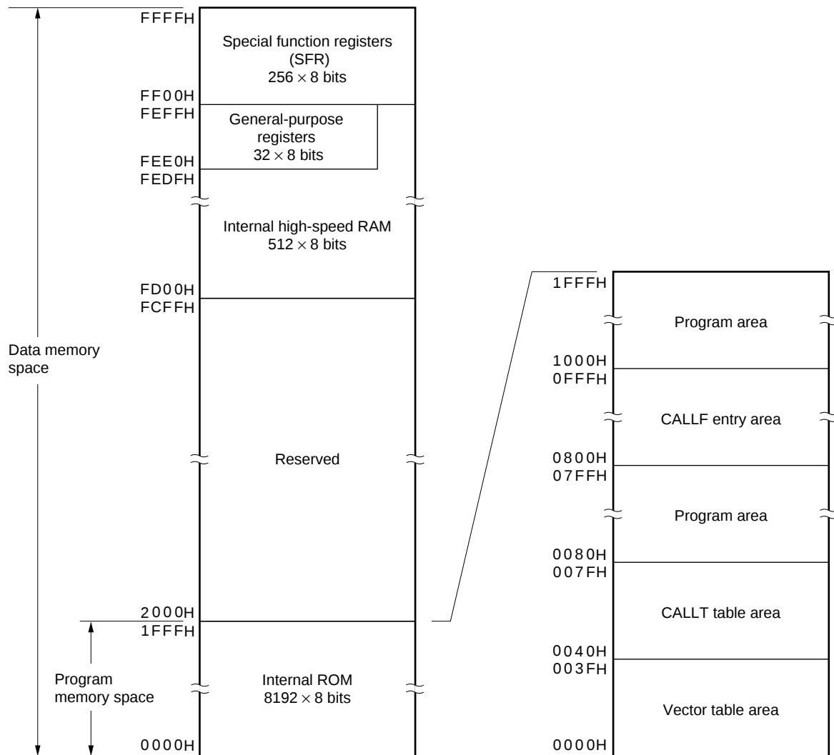
Figure 3-1. Memory Map ( \mu PD780131)
