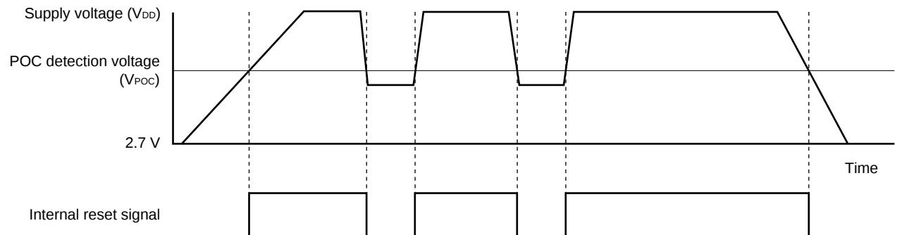
Figure 22-2. Timing of Internal Reset Signal Generation in Power-on-Clear Circuit
