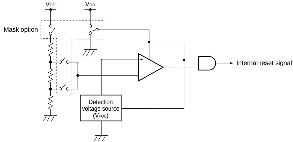
Figure 22-1. Block Diagram of Power-on-Clear Circuit
