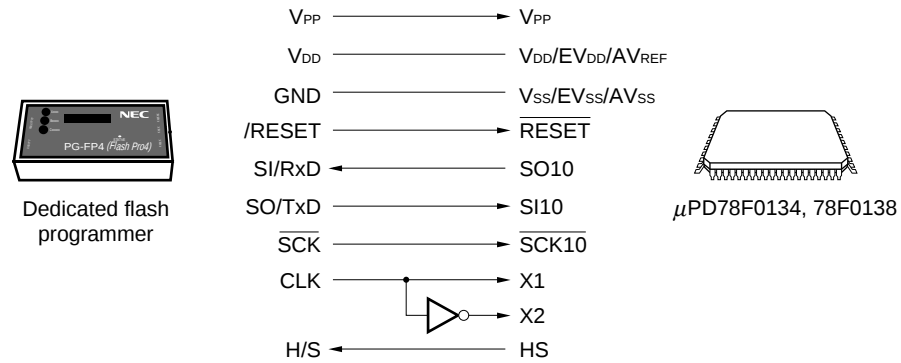
Figure 27-10. Communication with Dedicated Flash Programmer (CSI10 + HS)
