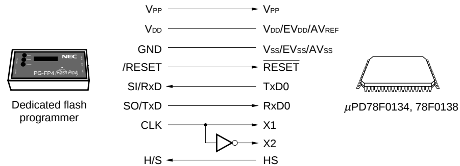
Figure 27-12. Communication with Dedicated Flash Programmer (UART0 + HS)
