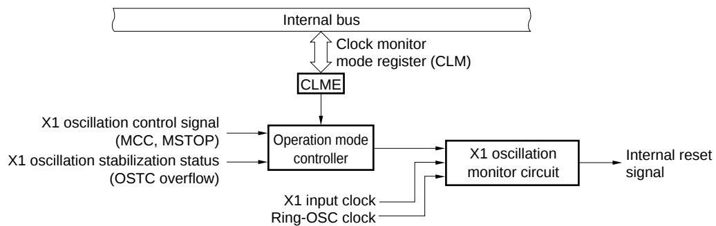
Figure 21-1. Block Diagram of Clock Monitor
