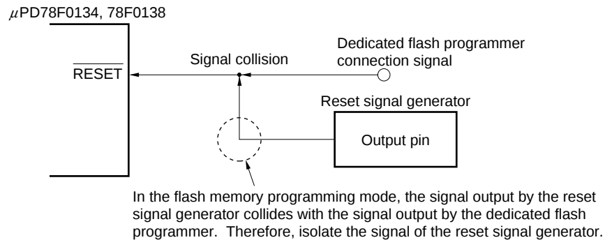
Figure 27-17. Signal Collision ( \overline{\text{RESET}} Pin)
