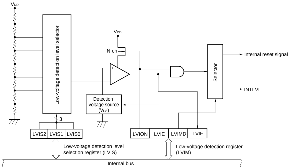
★ Figure 23-1. Block Diagram of Low-Voltage Detector
