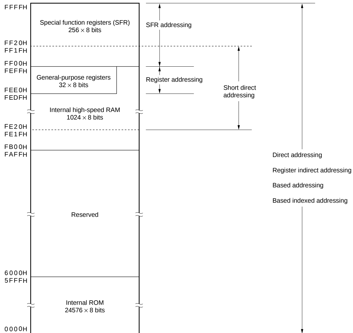
Figure 3-11. Correspondence Between Data Memory and Addressing ( \mu PD780133)
