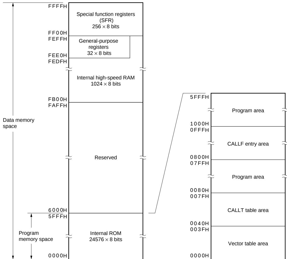
Figure 3-3. Memory Map ( \mu PD780133)
