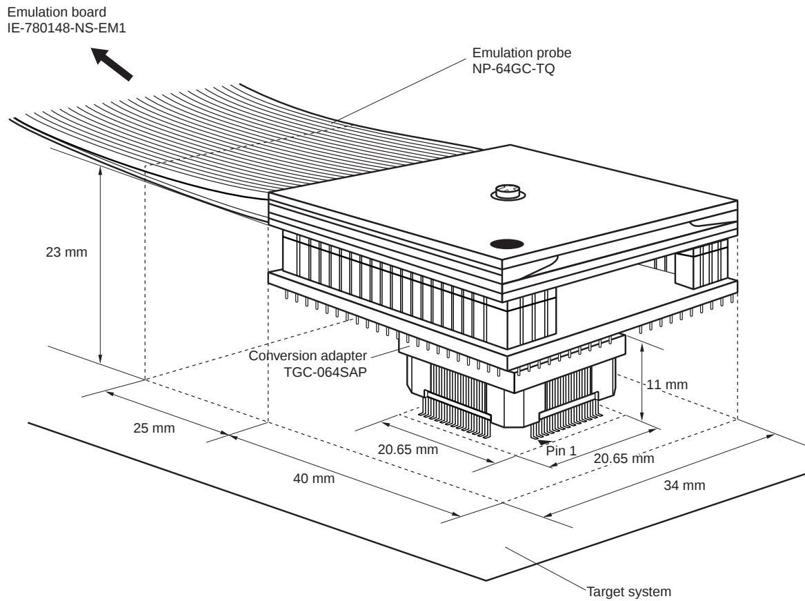
Figure B-4. Connection Conditions of Target System (When Using NP-64GC-TQ)
