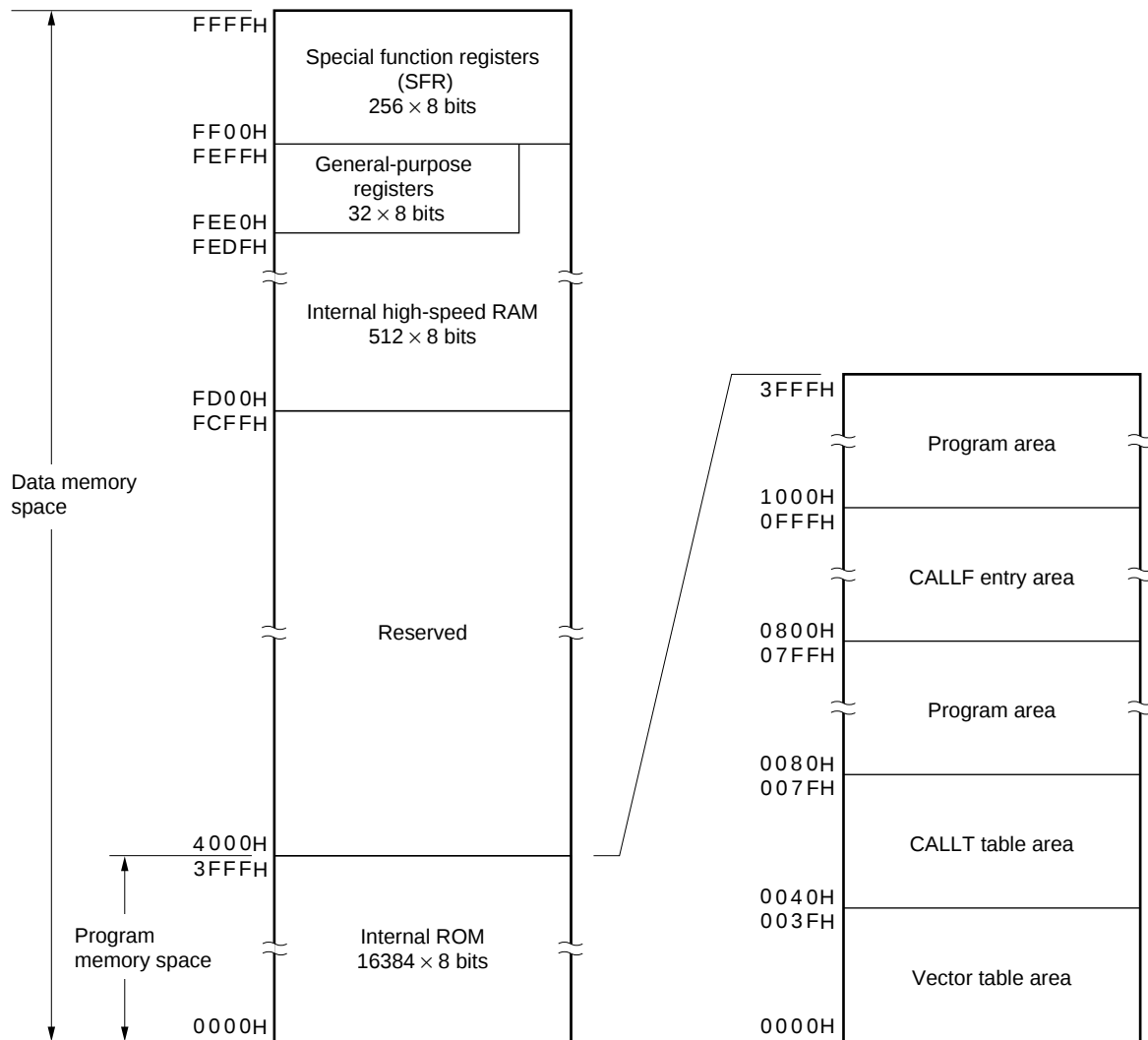
Figure 3-2. Memory Map ( \mu PD780132)
