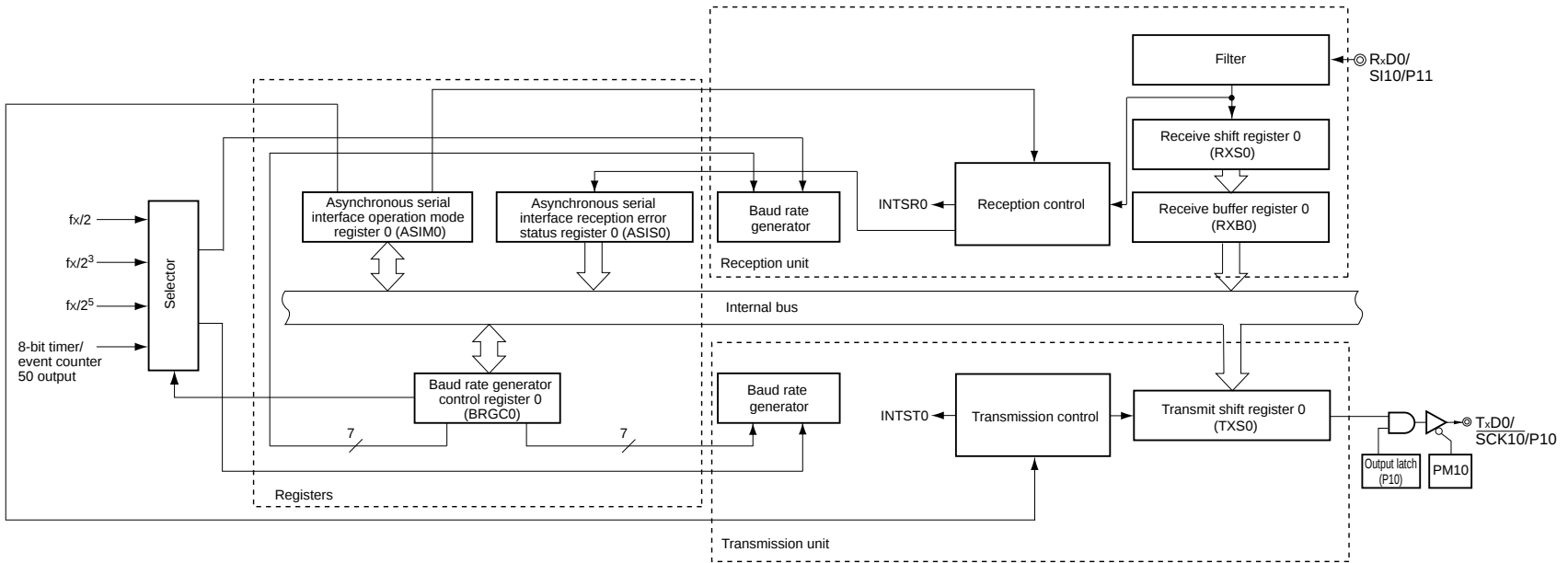
★ Figure 13-1. Block Diagram of Serial Interface UART0
