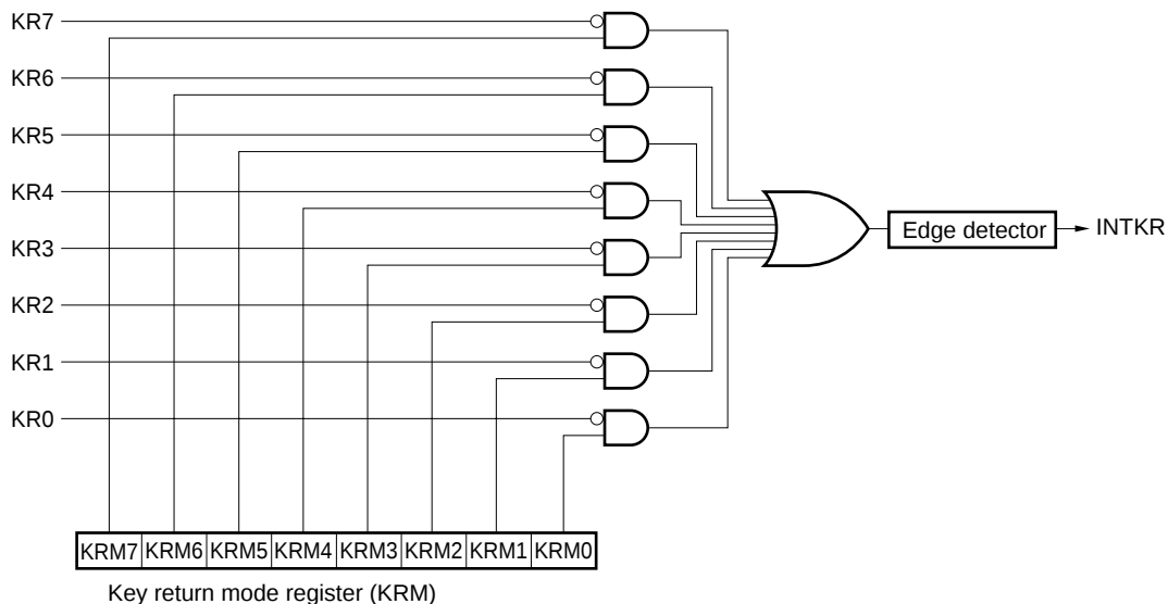
Figure 18-1. Block Diagram of Key Interrupt
