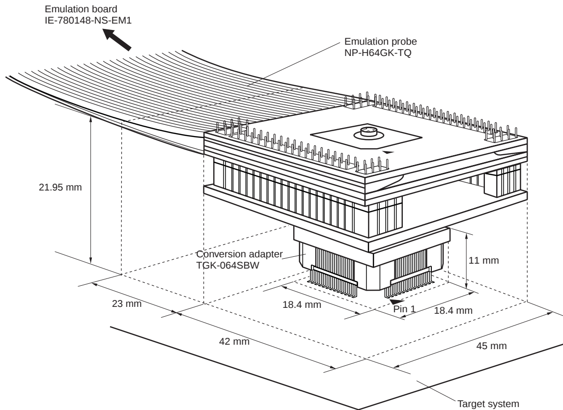
Figure B-7. Connection Conditions of Target System (When Using NP-H64GK-TQ)
