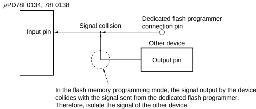
Figure 27-15. Signal Collision (Input Pin of Serial Interface)
