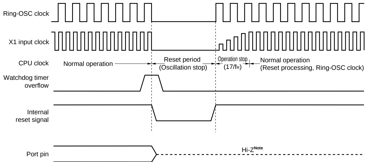
Figure 20-3. Timing of Reset Due to Watchdog Timer Overflow
