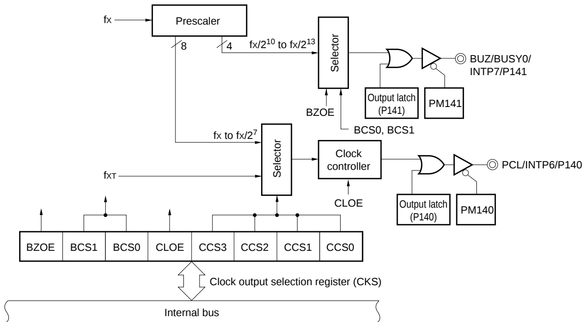
★ Figure 11-1. Block Diagram of Clock Output/Buzzer Output Controller
