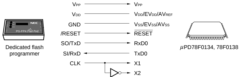
Figure 27-11. Communication with Dedicated Flash Programmer (UART0)
