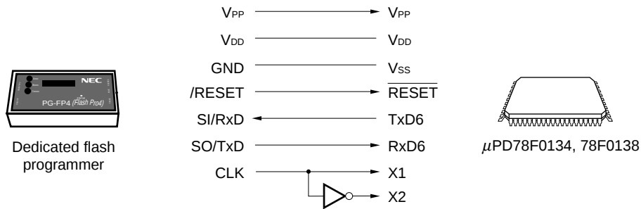
Figure 27-13. Communication with Dedicated Flash Programmer (UART6)
