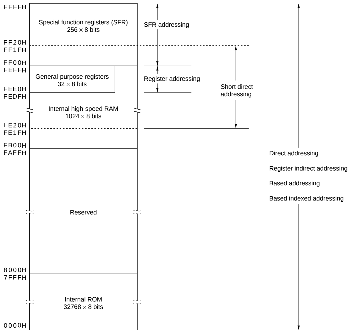
Figure 3-12. Correspondence Between Data Memory and Addressing ( \mu PD780134)
