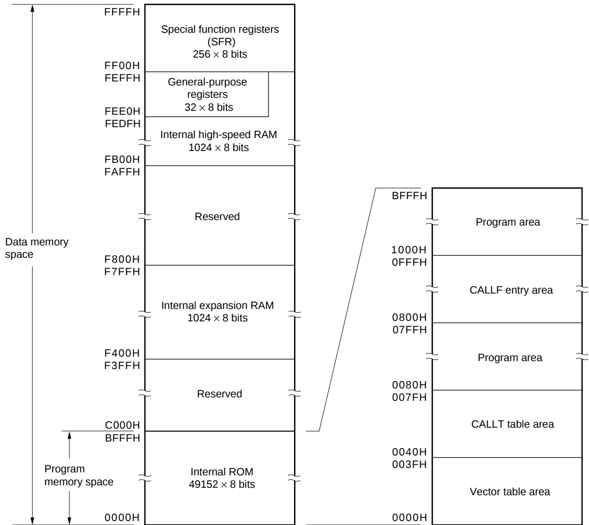
Figure 3-6. Memory Map ( \mu PD780136)
