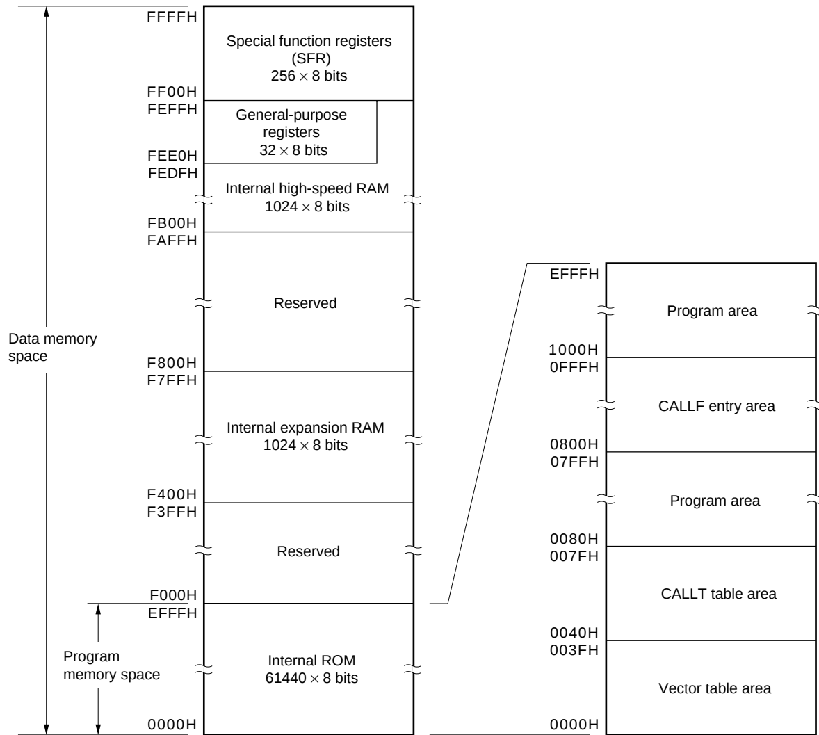
Figure 3-7. Memory Map ( \mu PD780138)
