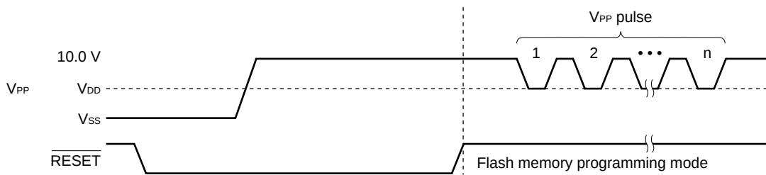
Figure 27-19. Flash Memory Programming Mode
