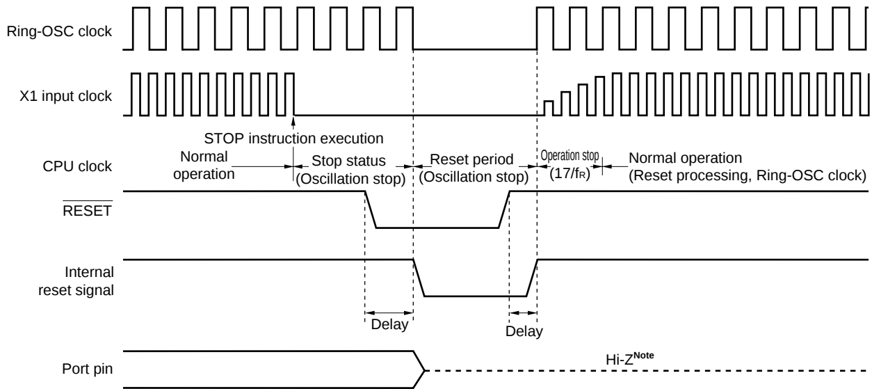
Figure 20-4. Timing of Reset in STOP Mode by \overline{\text{RESET}} Input
