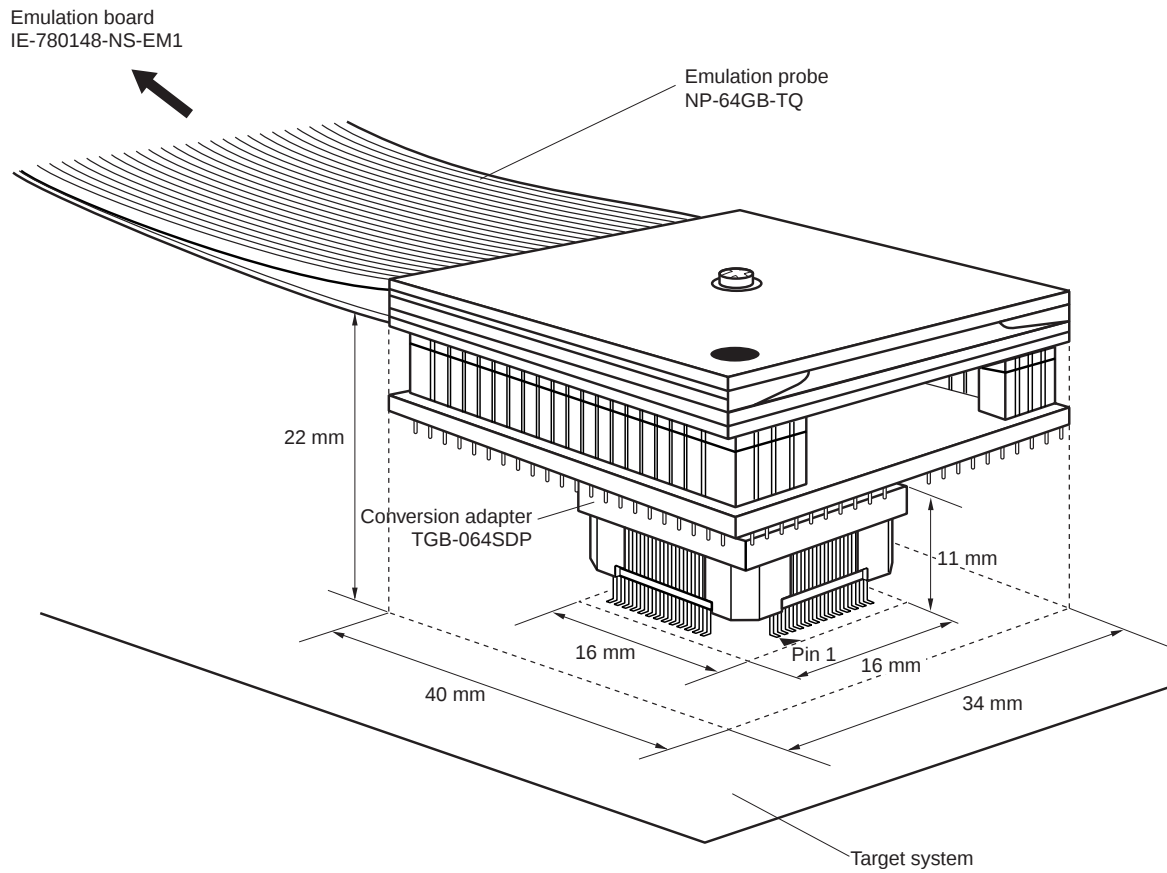
Figure B-2. Connection Conditions of Target System (When Using NP-64GB-TQ)
