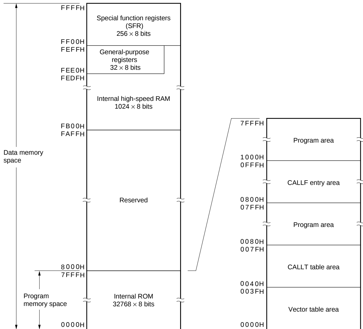
Figure 3-4. Memory Map ( \mu PD780134)
