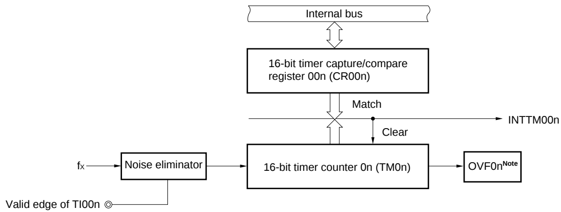
Figure 6-32. Configuration Diagram of External Event Counter
