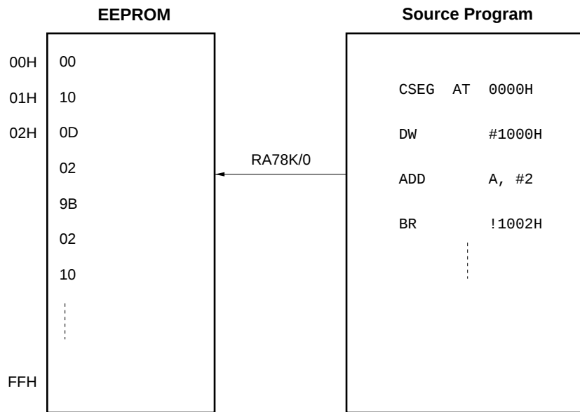
Figure 26-5. Example of Storing to EEPROM (When One Place Is Corrected)
