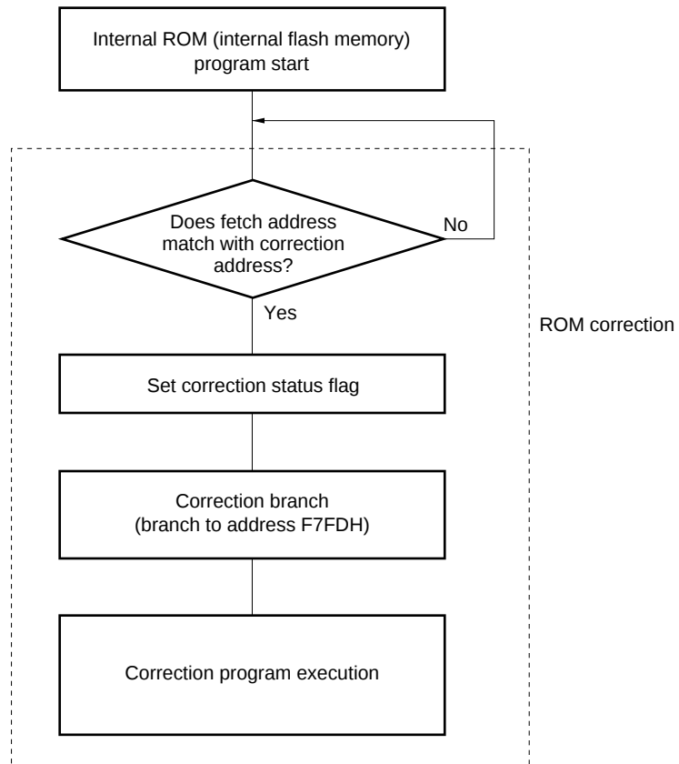
Figure 26-7. ROM Correction Operation
