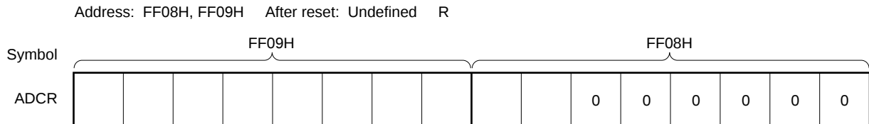
Figure 12-5. Format of A/D Conversion Result Register (ADCR)
