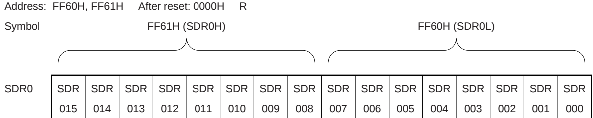
★ Figure 16-2. Format of Remainder Data Register 0 (SDR0)
