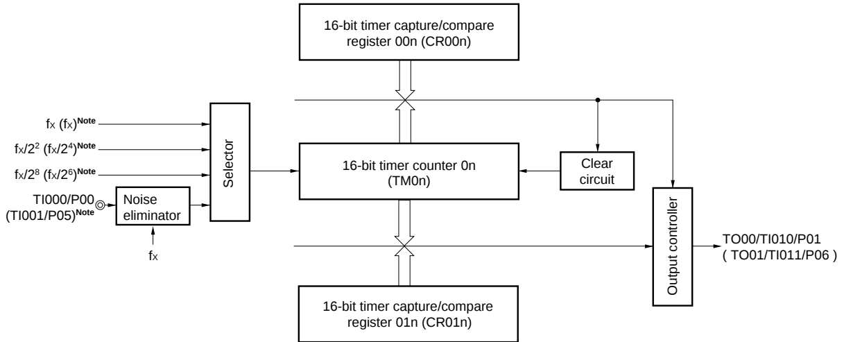
Figure 6-19. Configuration Diagram of PPG Output
