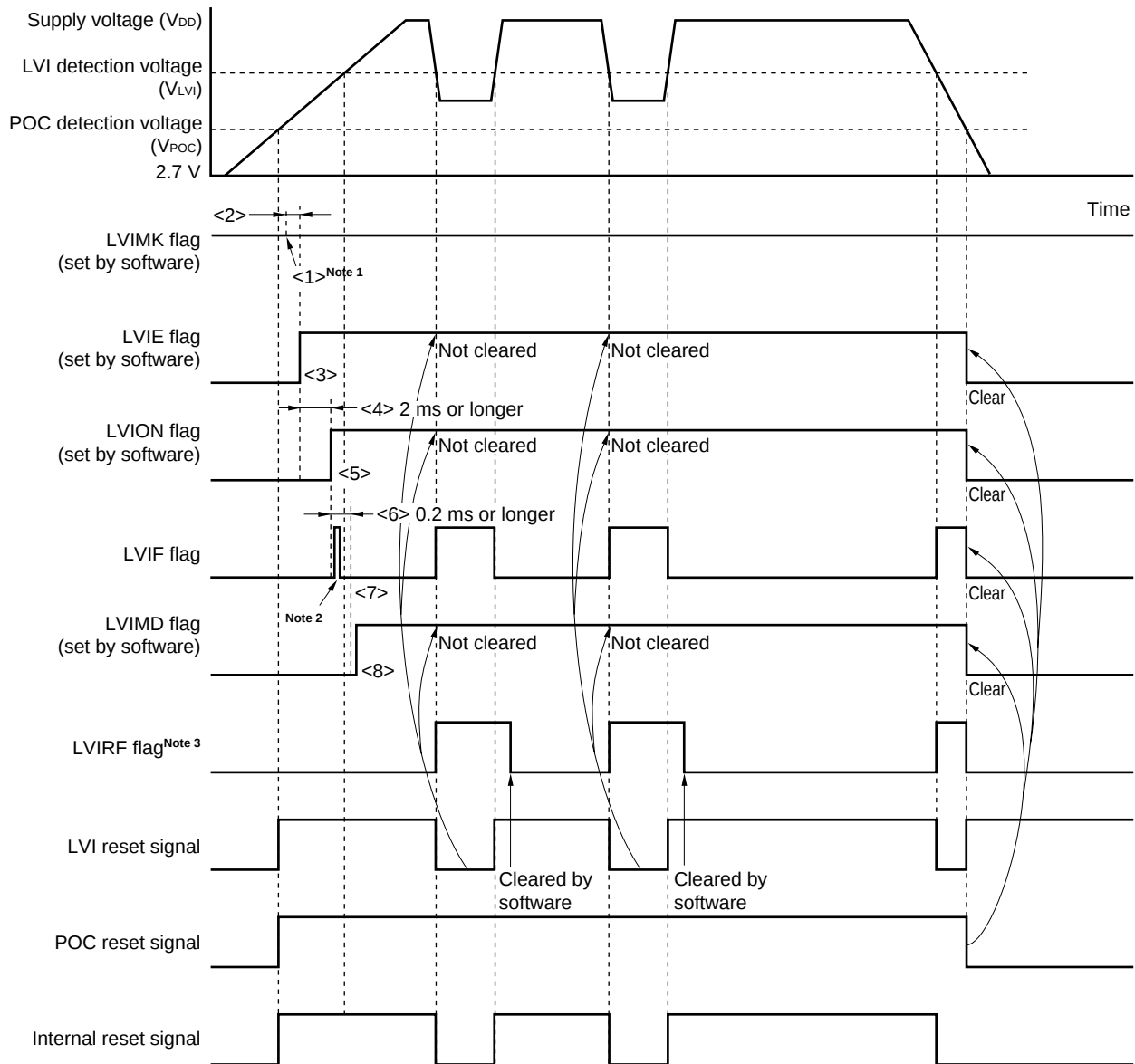
Figure 23-4. Timing of Low-Voltage Detector Internal Reset Signal Generation
