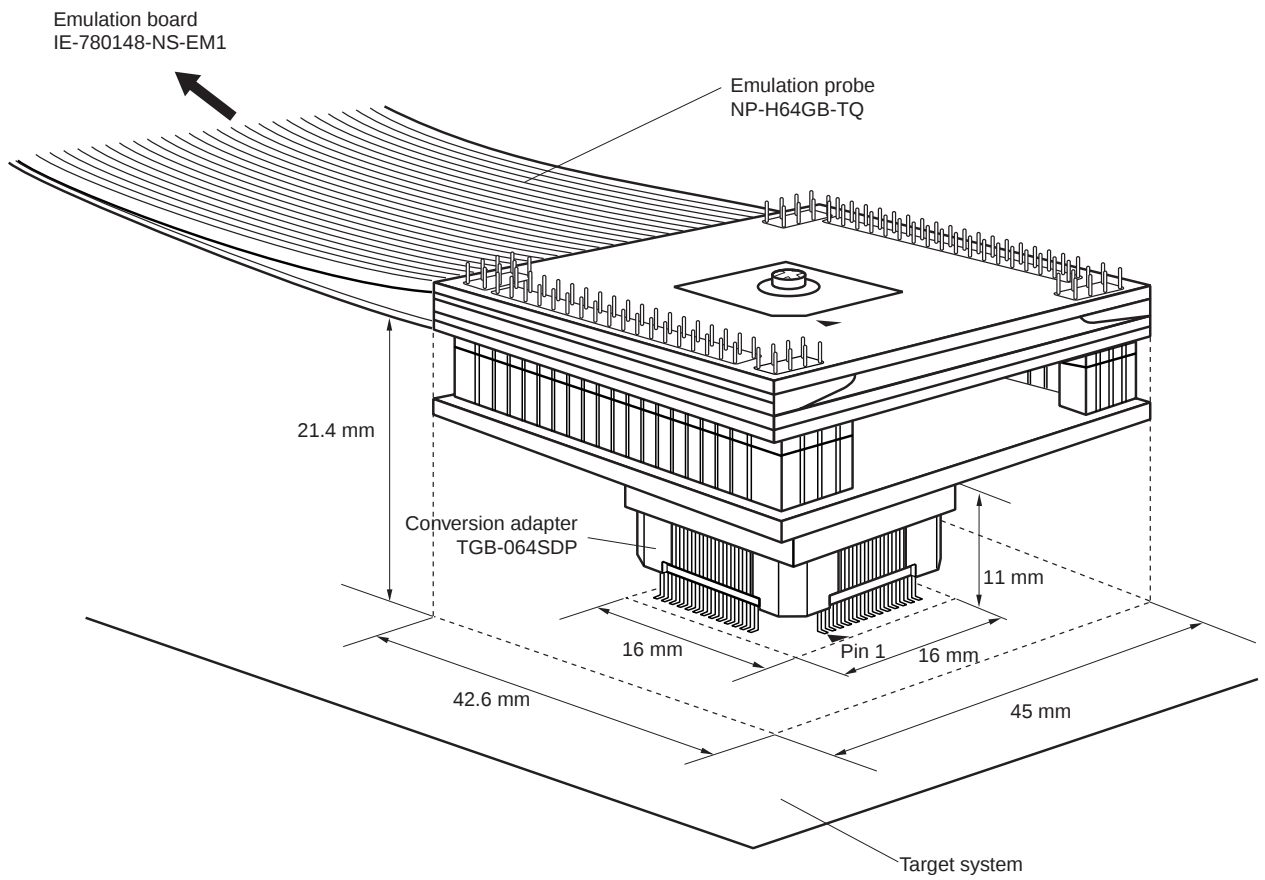
Figure B-3. Connection Conditions of Target System (When Using NP-H64GB-TQ)
