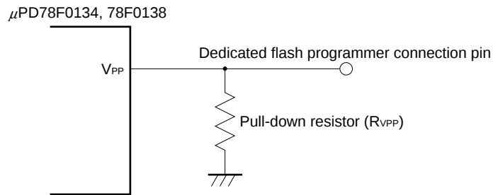
Figure 27-14. Example of Connection of V_{PP} Pin
