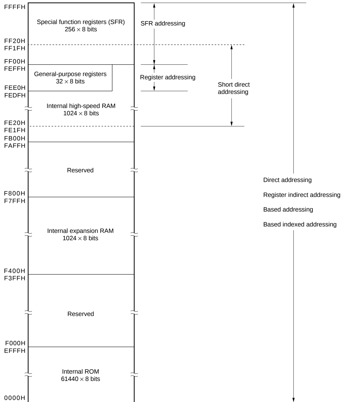
Figure 3-15. Correspondence Between Data Memory and Addressing ( \mu PD780138)
