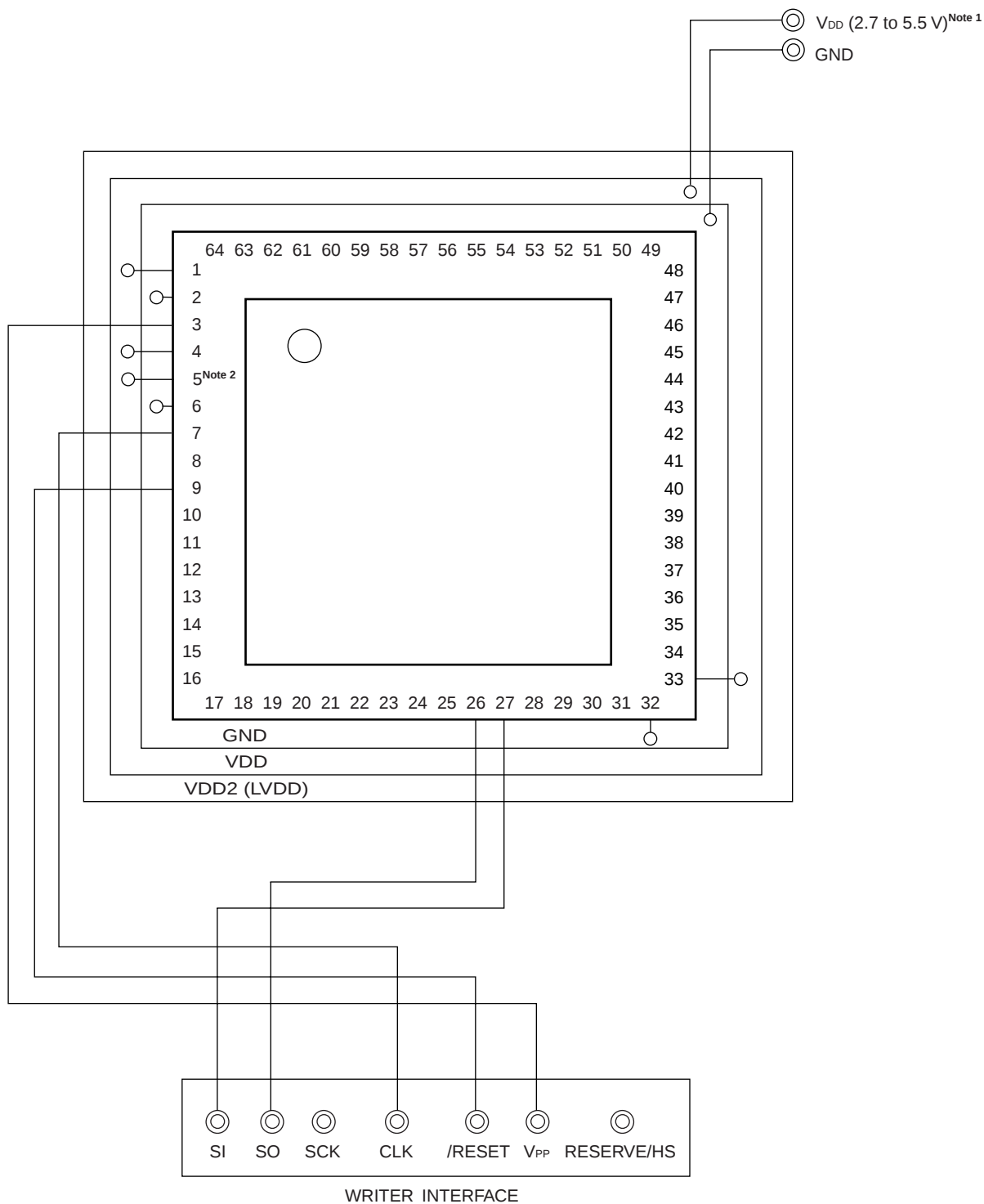
Figure 27-5. Example of Wiring Adapter for Flash Memory Writing in UART (UART0) Mode
