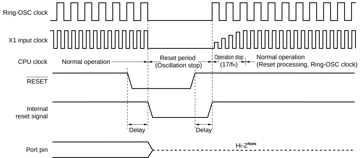
Figure 20-2. Timing of Reset by \overline{\text{RESET}} Input
