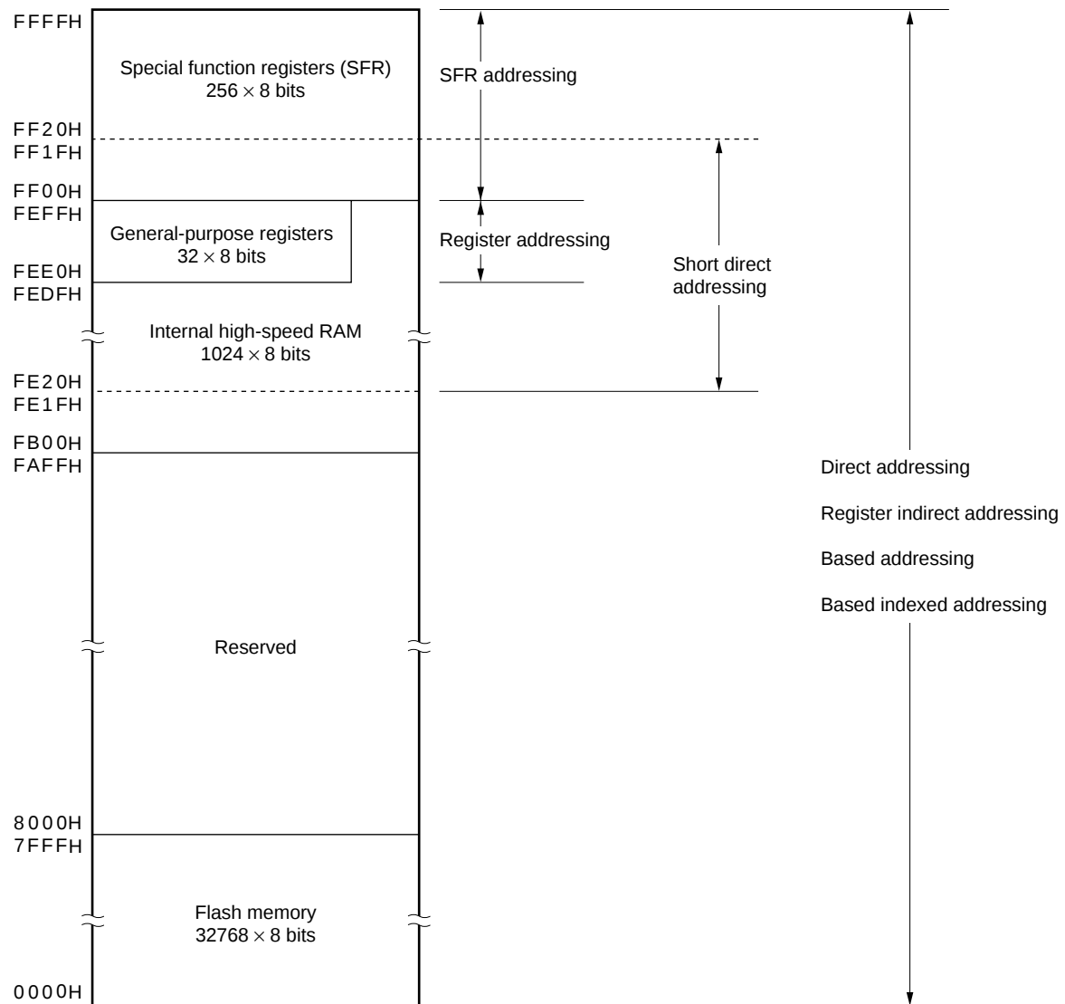
Figure 3-13. Correspondence Between Data Memory and Addressing ( \mu PD78F0134)
