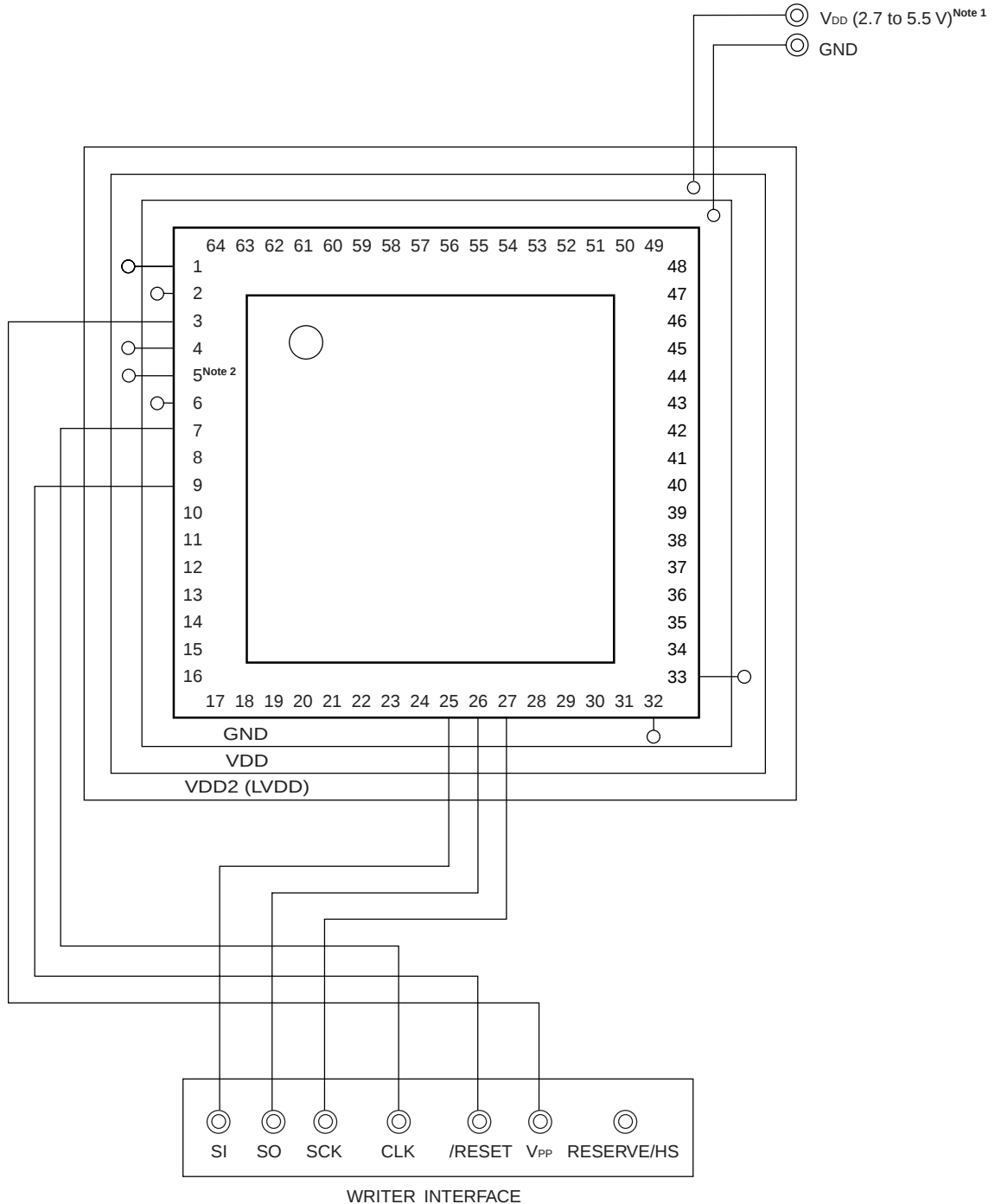
Figure 27-3. Example of Wiring Adapter for Flash Memory Writing in 3-Wire Serial I/O (CSI10) Mode
