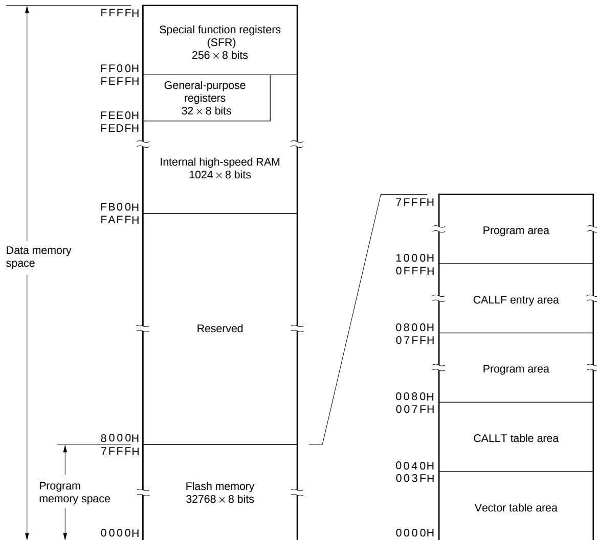
Figure 3-5. Memory Map ( \mu PD78F0134)
