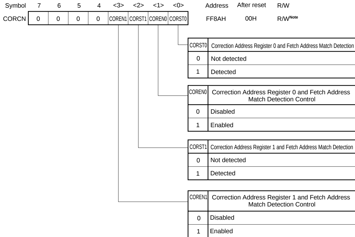
Figure 26-3. Format of Correction Control Register
