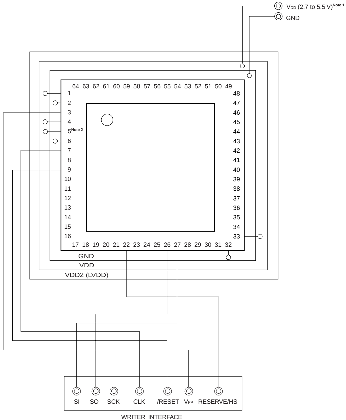
Figure 27-6. Example of Wiring Adapter for Flash Memory Writing in UART (UART0 + HS) Mode
