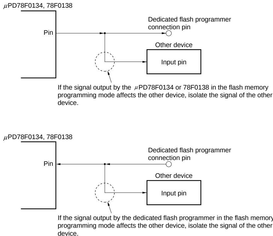
Figure 27-16. Malfunction of Other Device
