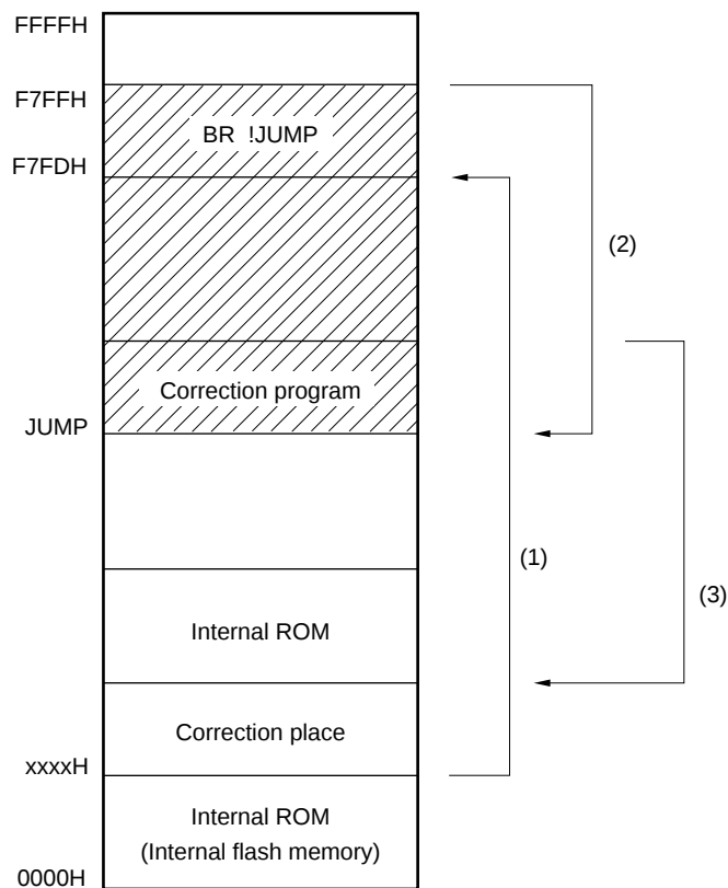
Figure 26-8. Program Transition Diagram (When One Place Is Corrected)
