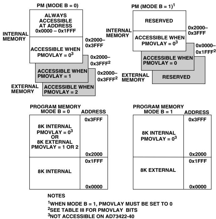
Figure 13. Program Memory Map
