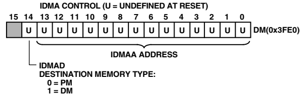
Figure 17. IDMA Control/OVLAY Registers
