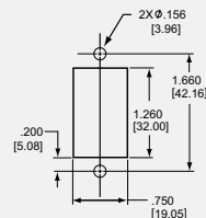
Mounting Detail Single, Two & Three Pole
