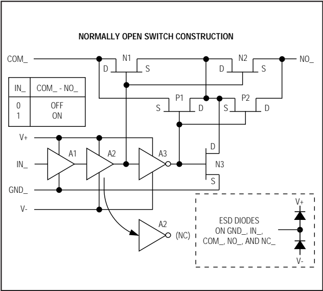
Figure 1. T-Switch Construction
