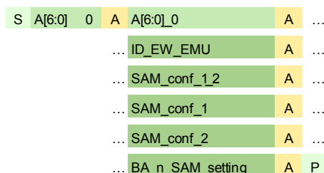
Figure 38. Emulate OTP bit without parity detection
