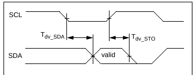
Figure 1-15. I²C I/O Timing
