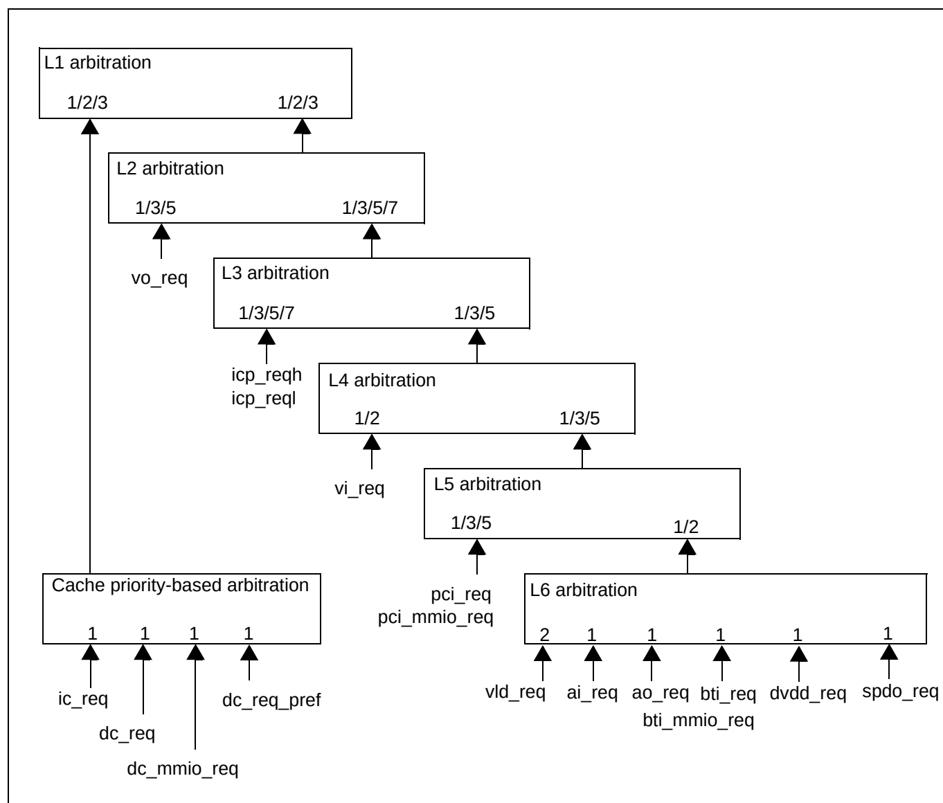
Figure 20-5. Arbitration architecture
