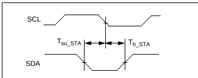
Figure 1-13. I²C I/O Timing
