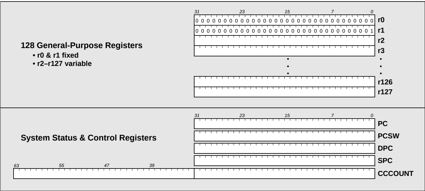
Figure 3-1. PNX1300 registers.
