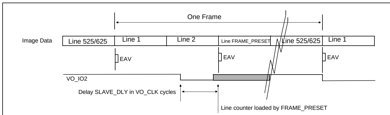
Figure 7-16. Genlock mode.
