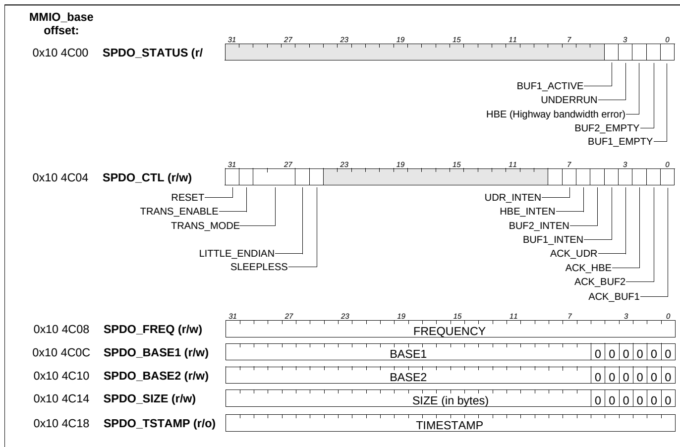
Figure 10-4. SPDO unit status/control field MMIO layout.
