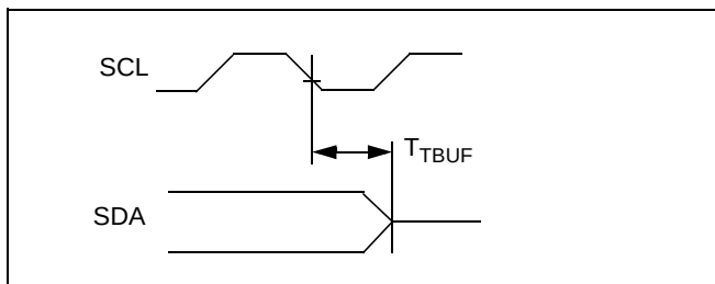
Figure 1-12. I²C I/O Timing
