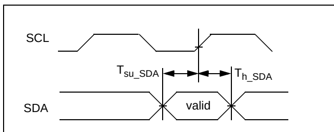
Figure 1-14. I²C I/O Timing
