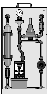
Fig. A: Portable dosing stations
