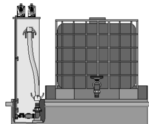
Fig. F: Dosing system with collecting pan and chemical feed tank
