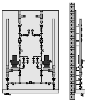
Fig. C: Panel mounted system
