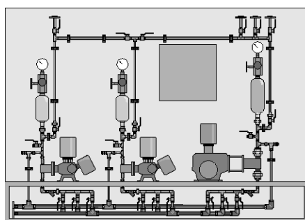
Fig. D: Frame mounted dosing systems
