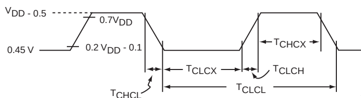
FIGURE 14-6: EXTERNAL CLOCK DRIVE WAVEFORM
