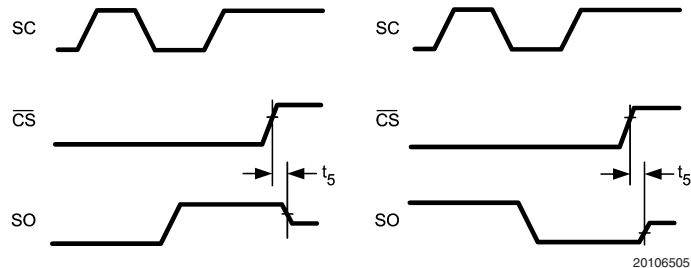
FIGURE 3. TRI-STATE Data Output Timing Diagram
