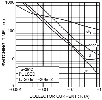
Fig.6 Switching time
