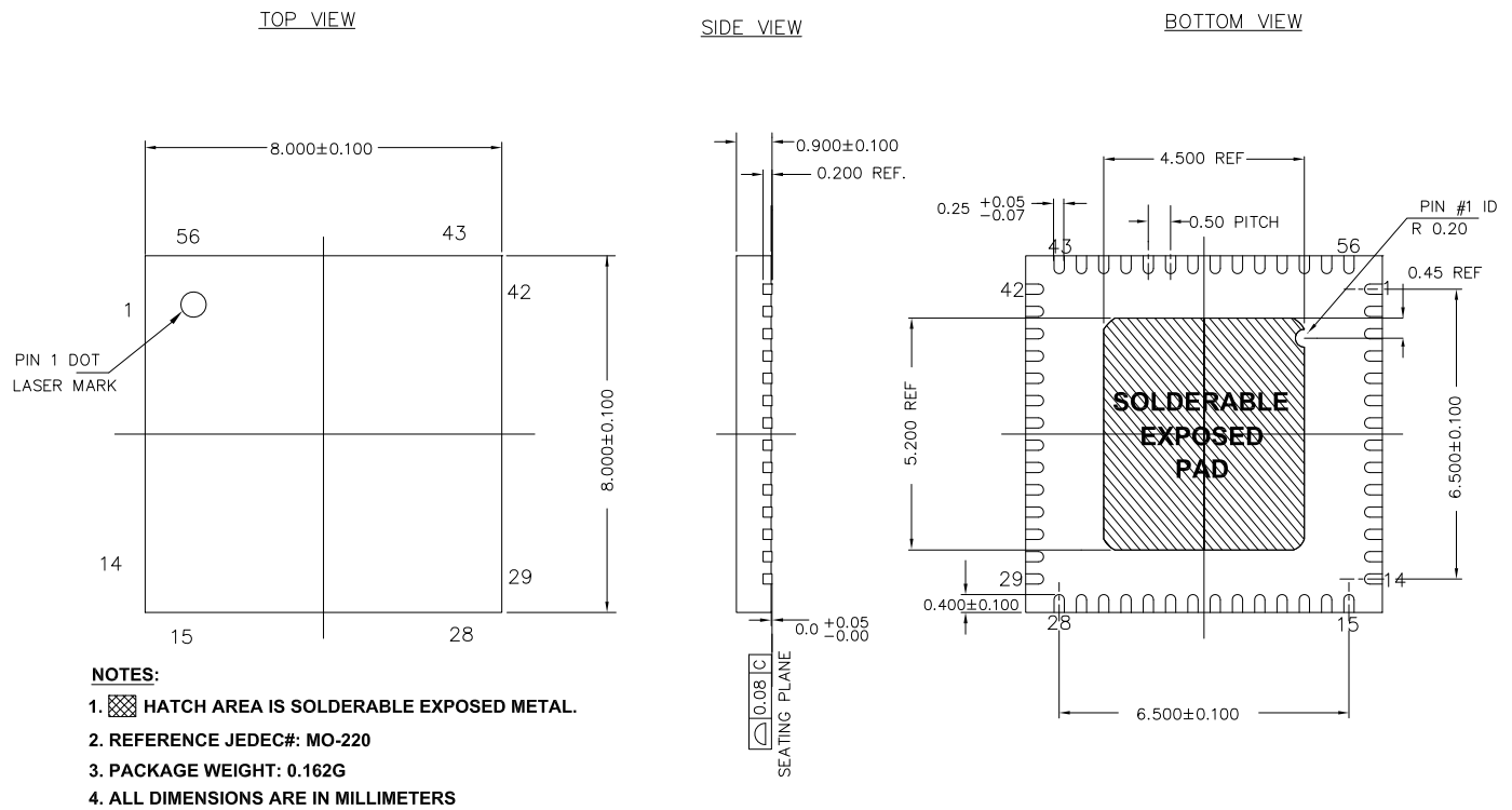
Figure 11-3. 56-Pin QFN 8 × 8 mm Sawn Version (001-53450)
