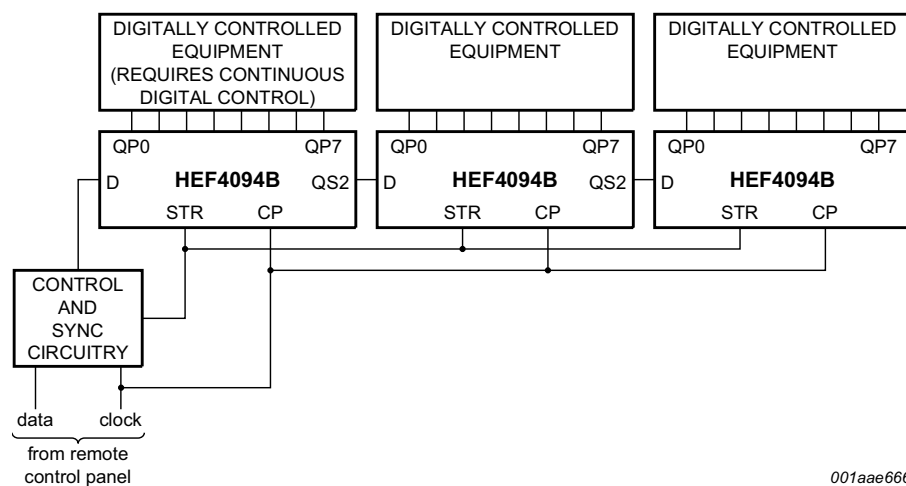
Fig 11. Remote control holding register
