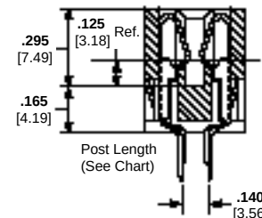
Flow Solder Post .140 [3.56] Row-to-Row Spacing
