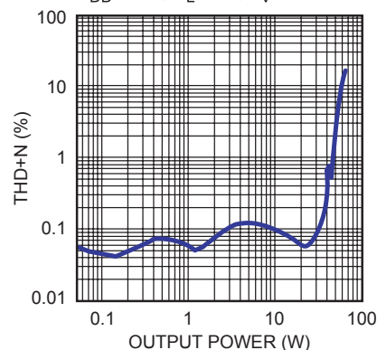
THD+N vs. Output Power V_{DD} = 24V , R_L = 6\Omega , A_V = 30
