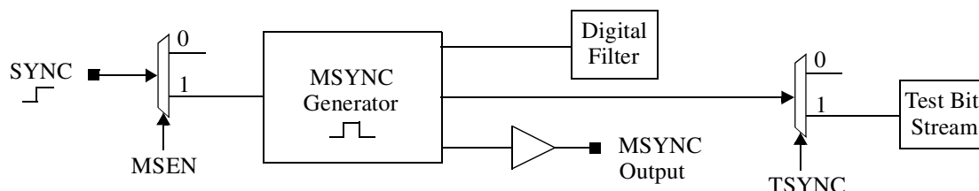
Figure 13. Synchronization Block Diagram
