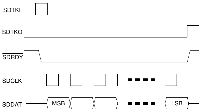
Figure 35. SD Port Transaction
