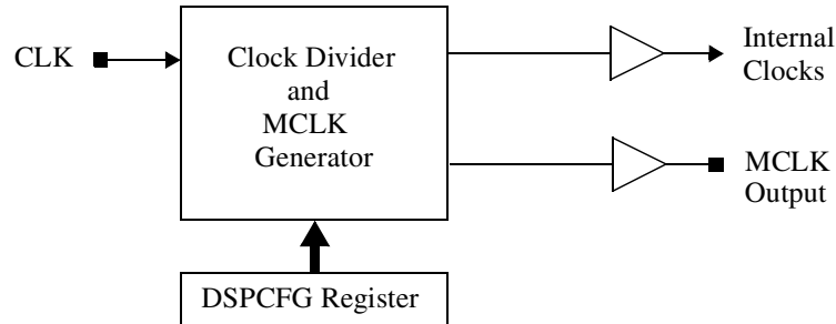
Figure 12. Clock Generation Block Diagram
