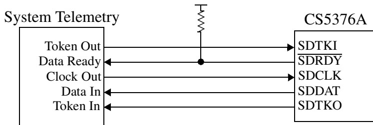
Figure 33. Serial Data Port Block Diagram
