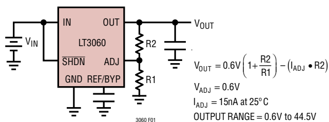
Figure 1. Adjustable Operation
