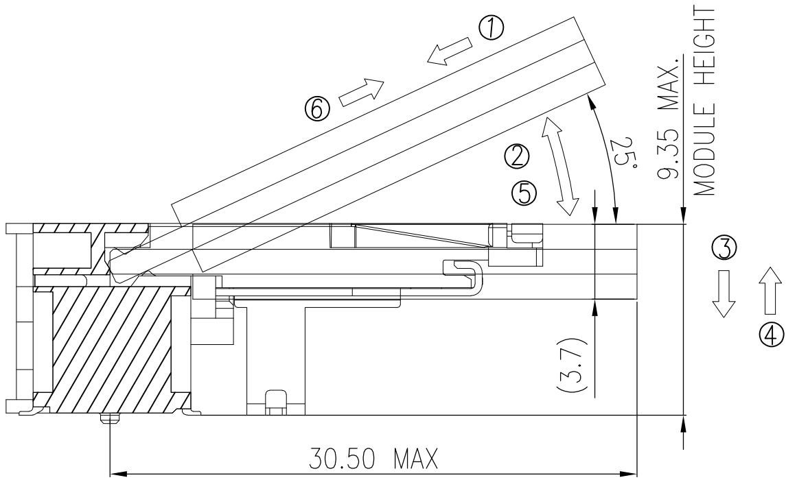
MATING/UNMATING VIEW
