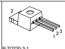
P-TO220-3-1
