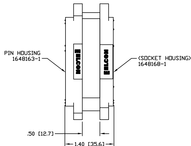
MATED CONDITION
