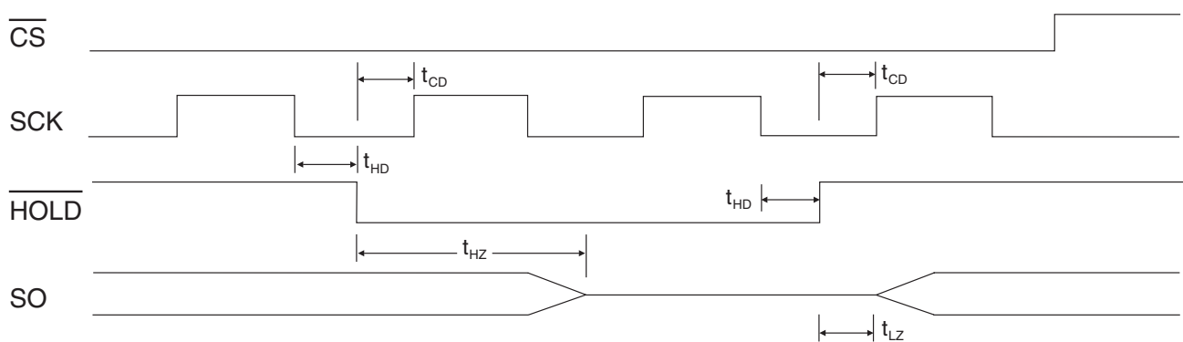
Figure 5-9. HOLD Timing
