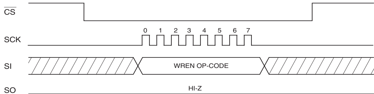
Figure 5-2. WREN Timing
