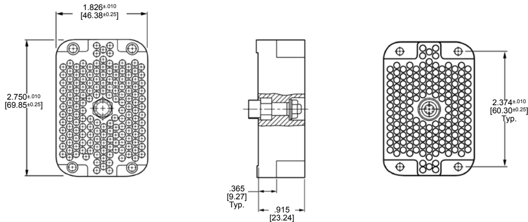
Receptacle Housing Phenolic Part No. 202800-2 Diallyl Phthalate Part No. 202800-1
