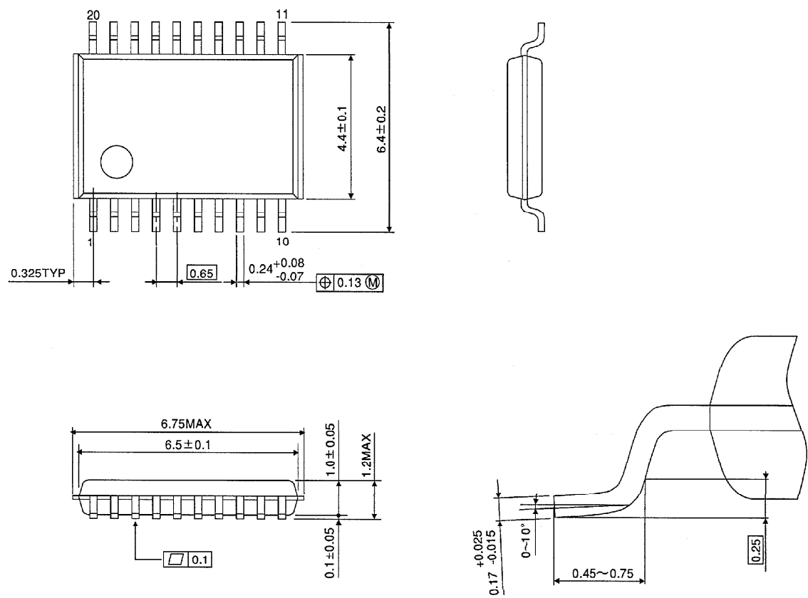
OUTLINE DRAWING TSSOP20-P-0044-0.65
